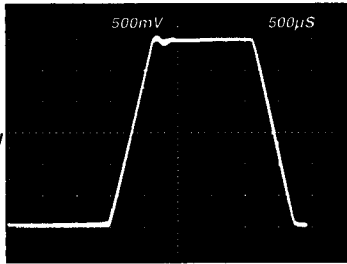
MAX406/MAX407/MAX418 LARGE-SIGNAL TRANSIENT RESPONSE
