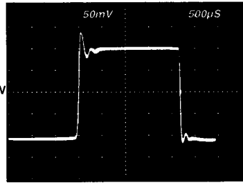
MAX406/MAX407/MAX418 SMALL-SIGNAL TRANSIENT RESPONSE
