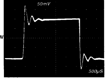
MAX406 (DECOMPENSATED MODE) SMALL-SIGNAL TRANSIENT RESPONSE
