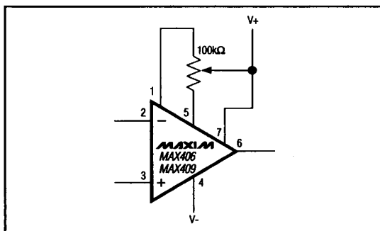
Figure 1. Offset-Voltage Adjustment
