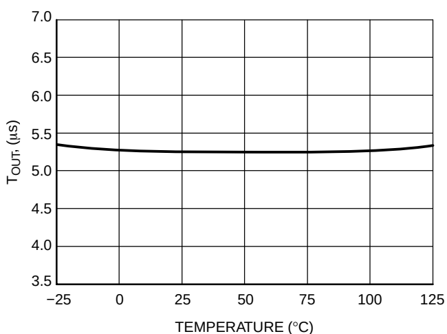
Figure 14. Demagnetization Detection Timeout versus Temperature
