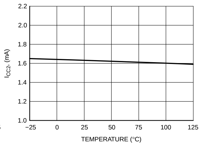
Figure 6. Current Consumption (1.0 nF Load) versus Temperature
