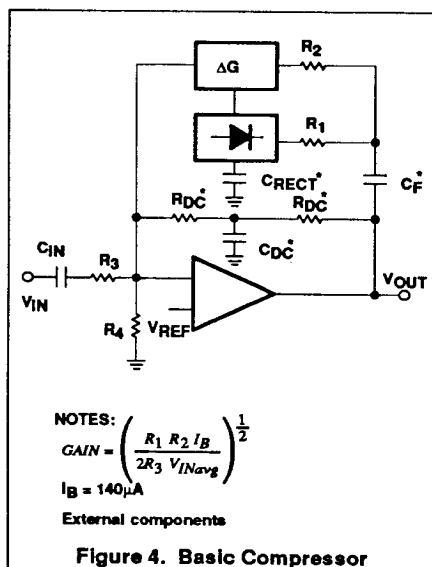
Figure 4. Basic Compressor
