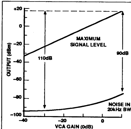
Figure 12. Dynamic Range of NE570
