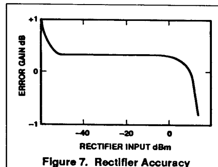
Figure 7. Rectifier Accuracy
