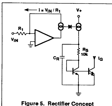
Figure 5. Rectifier Concept
