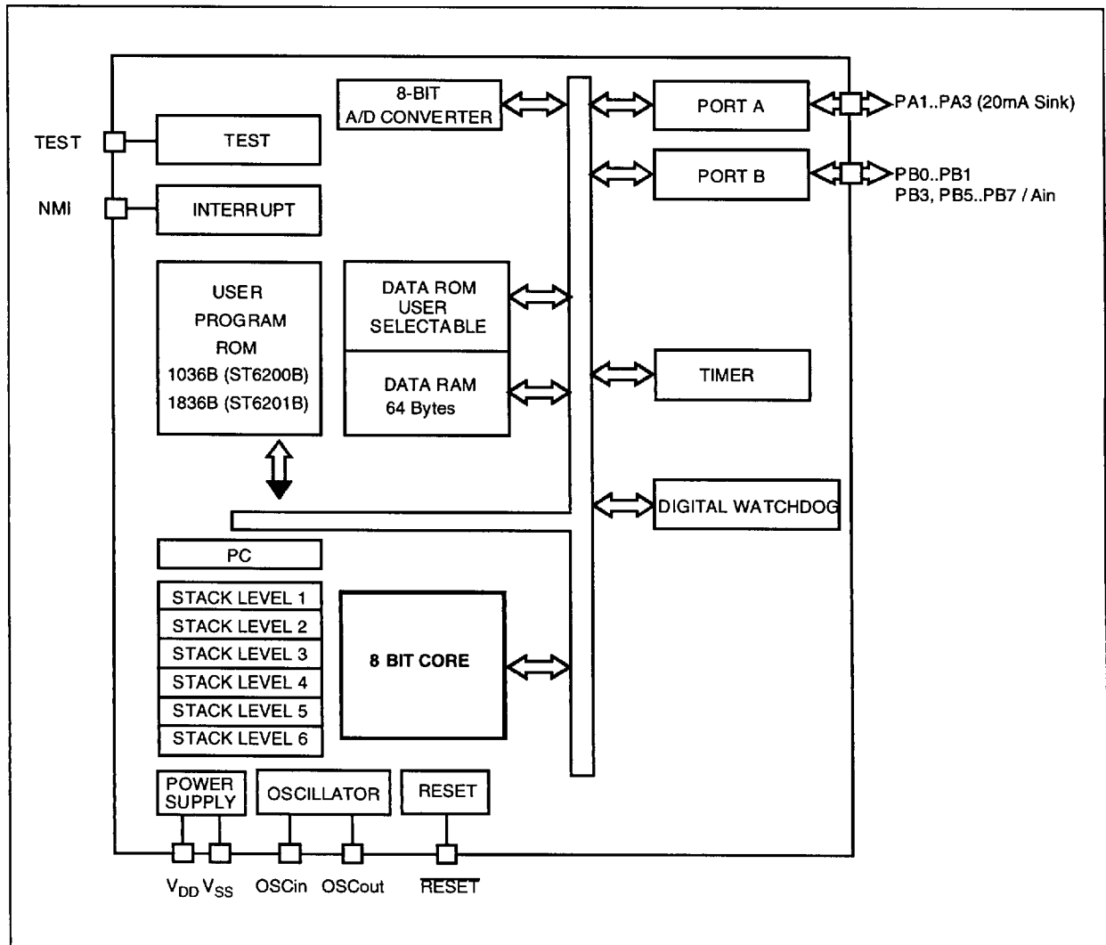
Figure 1. Block Diagram
