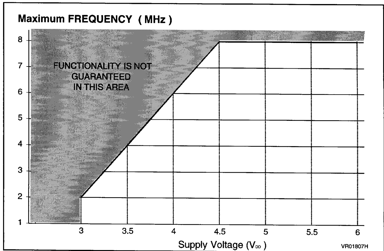
Figure 5. Maximum Operating FREQUENCY ( f_{MAX} ) Versus SUPPLY VOLTAGE ( V_{DD} )
