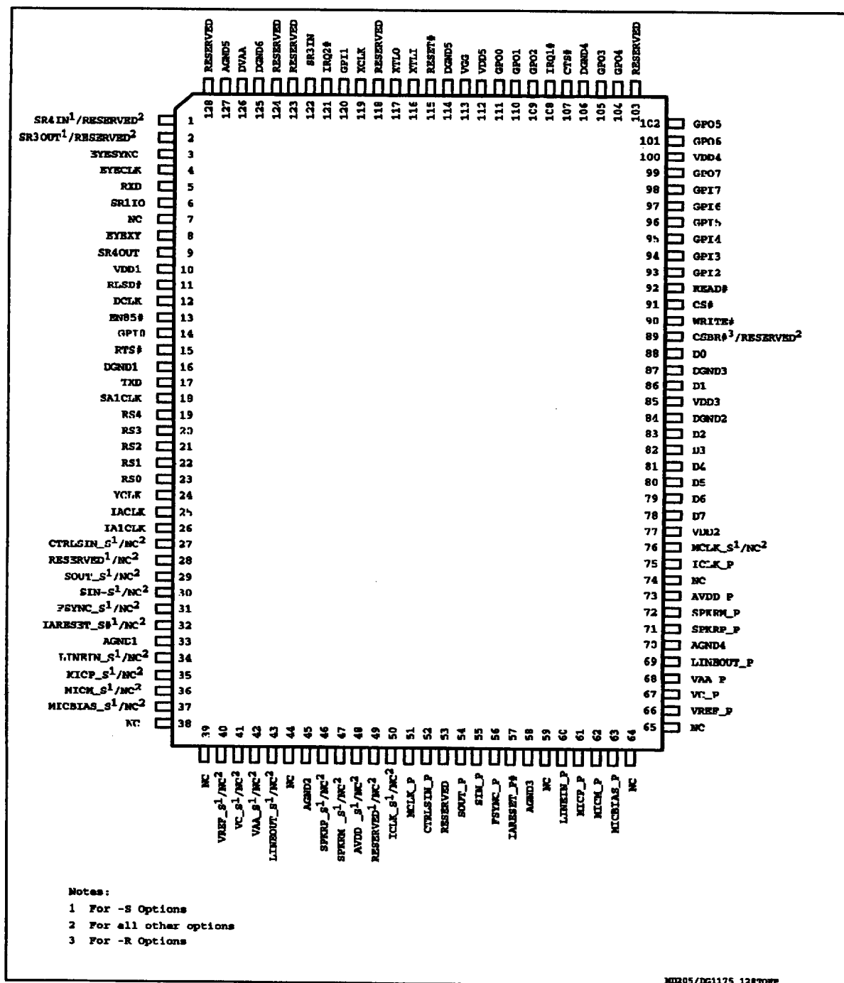
Figure 4. Pin Signals - 128-Pin TQFP
