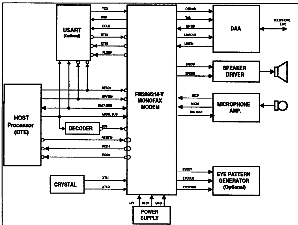
Figure 2. Modem Functional Interconnect Diagram (Fax and DTAM)
