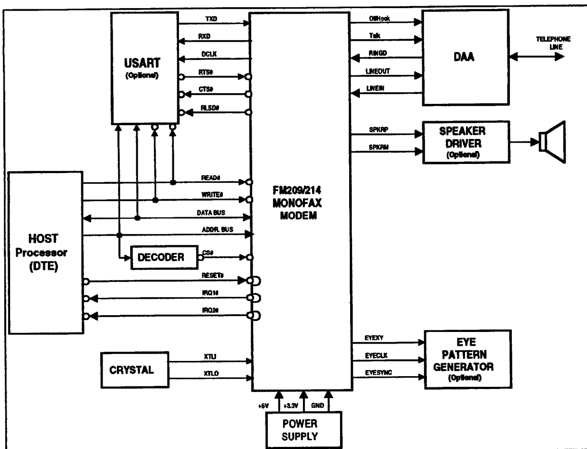
Figure 1. Modem Functional Interconnect Diagram (Fax)
