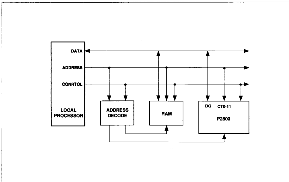
Fig. 10 Memory mapped P2800 system
