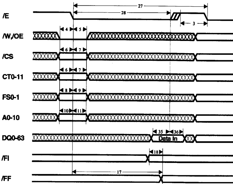
Fig. 7 Memory write cycle
