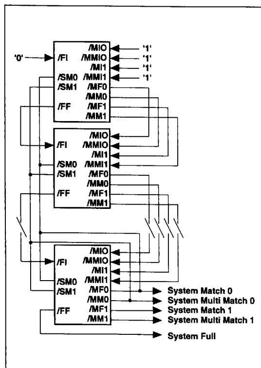
Fig.3 Vertically cascaded P2800 system
