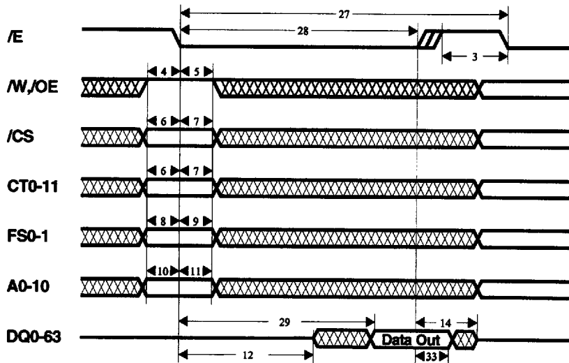
Fig. 6 Memory read cycle
