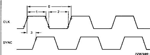
Fig. 4.3-5 Synchronization timing.
