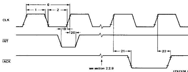
Fig. 4.3-3 Interrupt timing.
