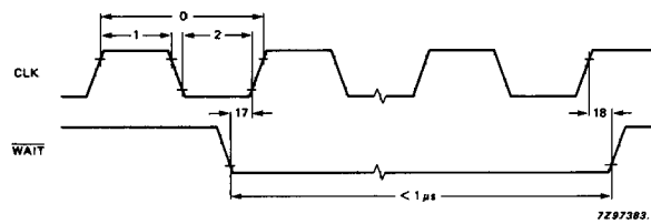
Fig. 4.3-8 \overline{\text{WAIT}} signal timing.
