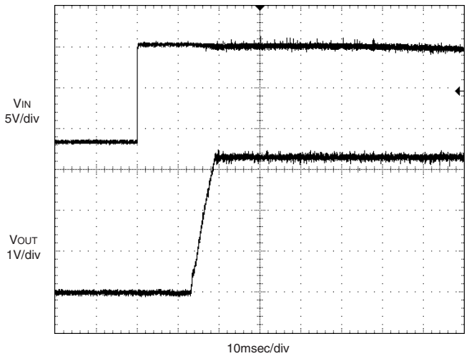
D12 Models, Start-up from V IN (Full load, using specified output capacitor.)
