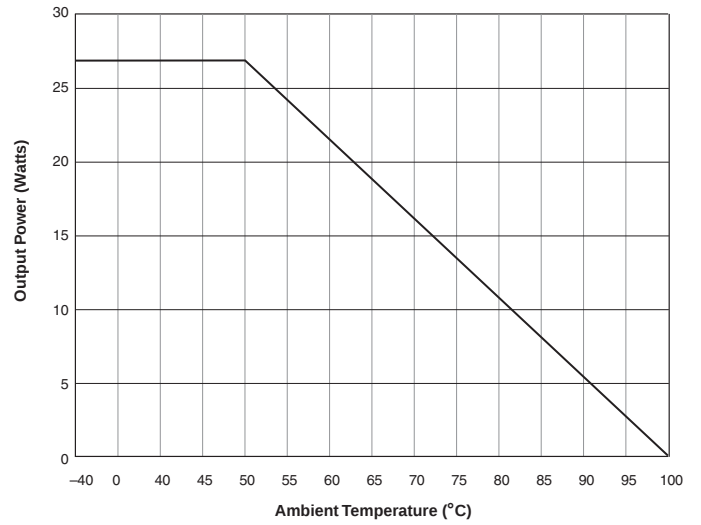
UNR-3.3/10-D5T/D5SM Output Power vs. Ambient Temperature, No Air Flow
