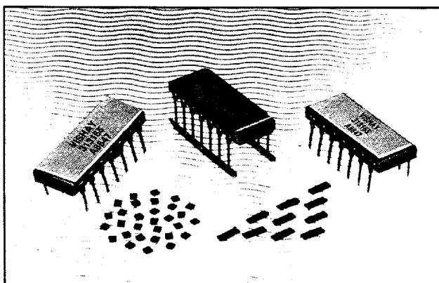
14 pins on a 0.300" pin spacing — can contain up to 30 V5X5 resistor chips.
