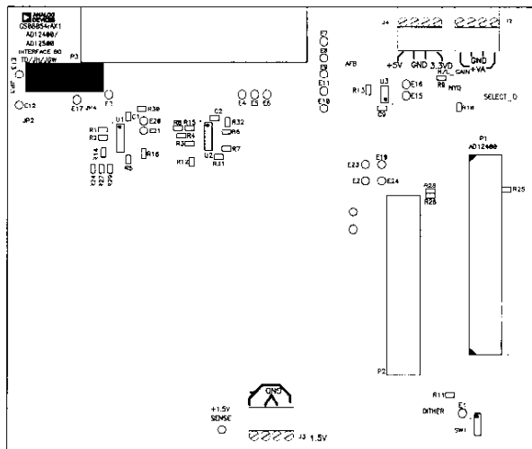
Figure 32. Top Silkscreen
