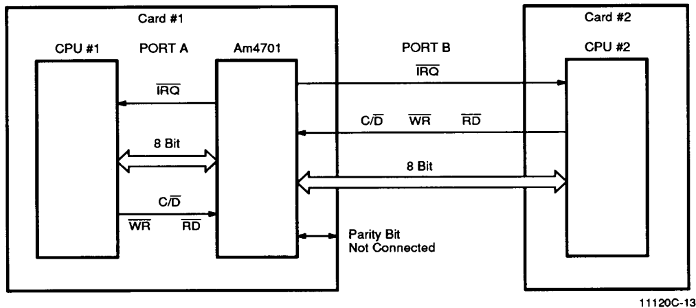
Figure 1. CPU-CPU Communication
