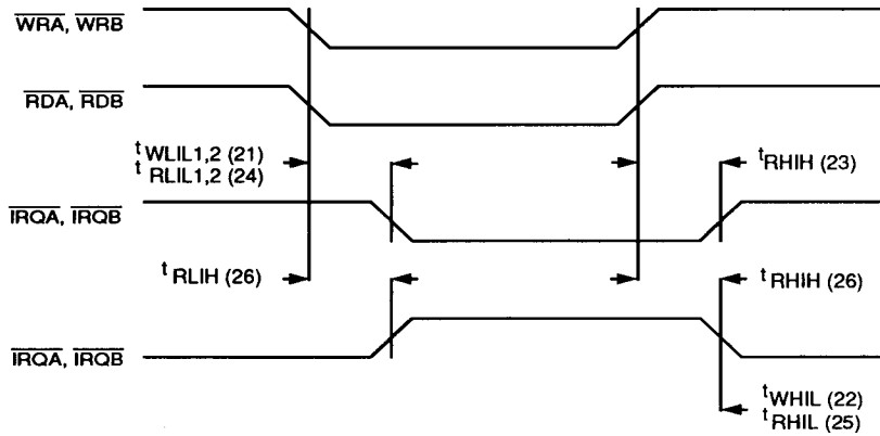
IRQ Timing
