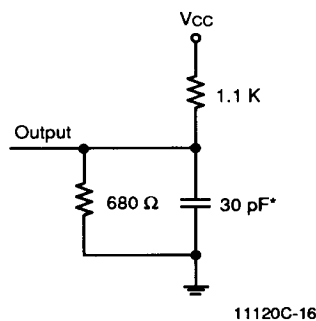
AC Test Load
