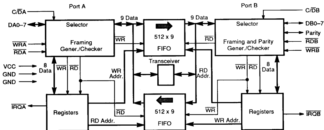
2-512 x 9 BiFIFO
