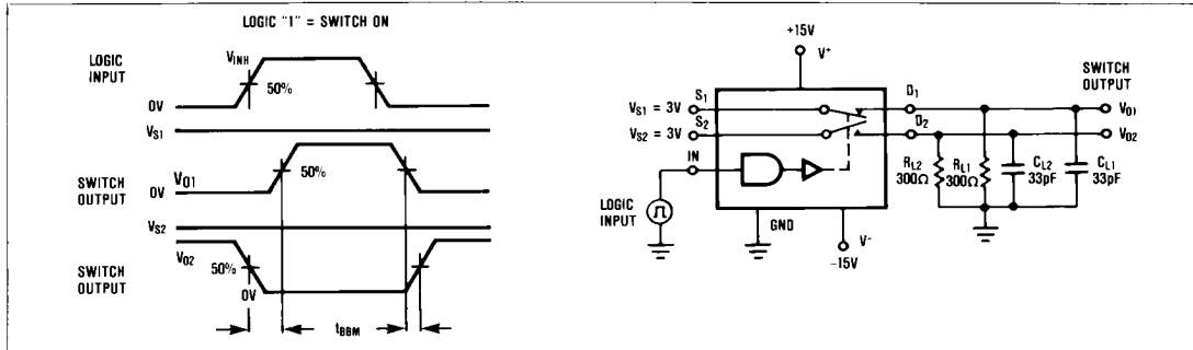
Figure 2. Break-Before-Make Time Test Circuit SPDT DG305(A), DG307(A).
