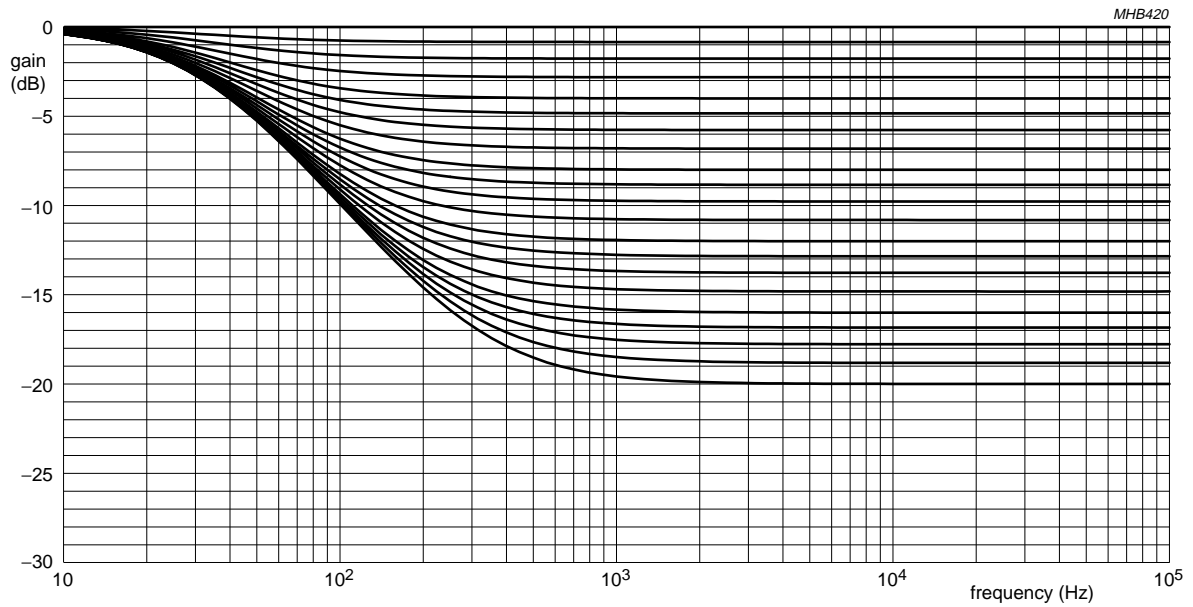
Fig.14 Loudness with bass boost only without influence of coupling capacitors C_{KVL} and C_{KVR} .
