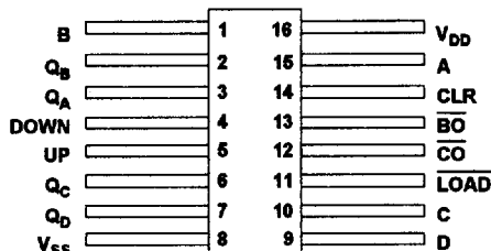
16-Lead Flatpack Top View
