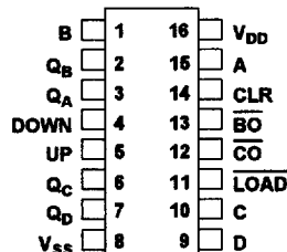
16-Lead Flatpack Top View
