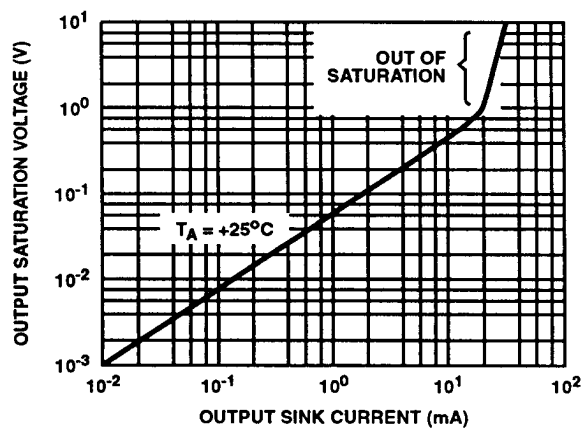
FIGURE 7. OUTPUT SATURATION VOLTAGE vs OUTPUT SINK CURRENT
