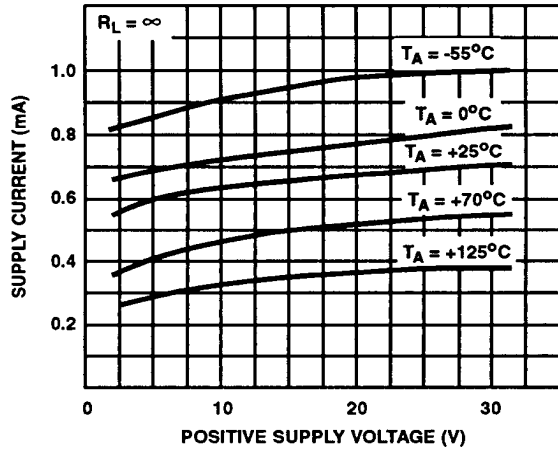
FIGURE 1. SUPPLY CURRENT vs SUPPLY VOLTAGE
