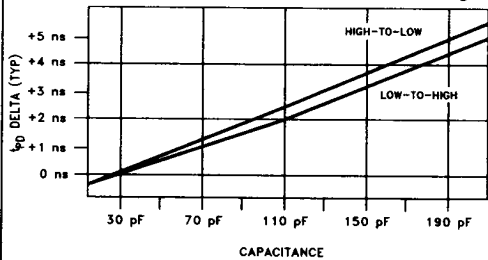
iPLD910 t_{PD} Derating vs Capacitive Loading
