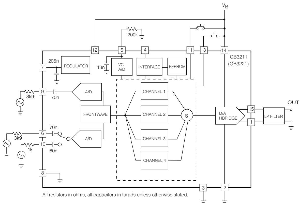
Figure 1: Test Circuit
