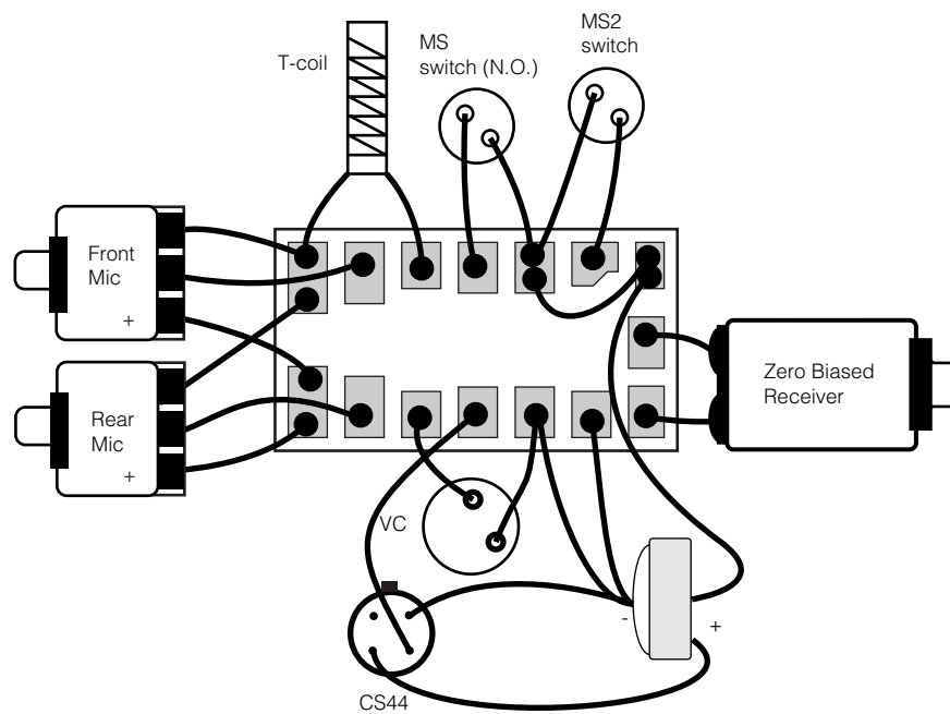
Figure 3: Assembly Diagram
