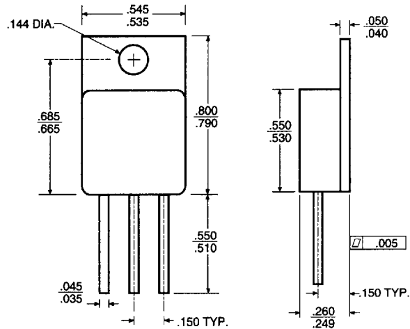
TO-254 AA Package
