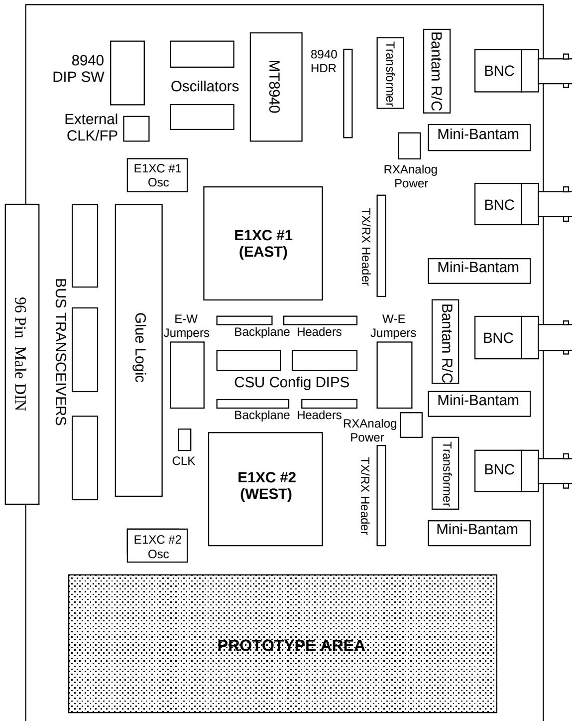
Figure 3: Board Layout
