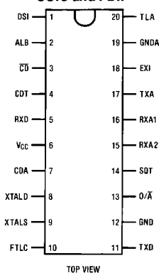
Pin Assignments for SOIC and PDIP
