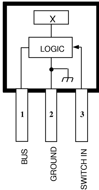
Dwg. PH-005
