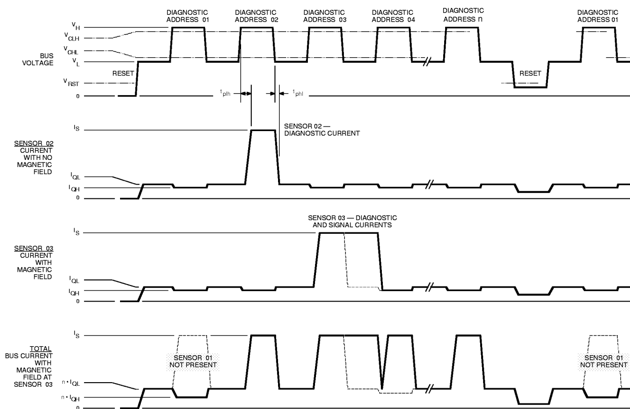
FIGURE 1 BUS TIMING
