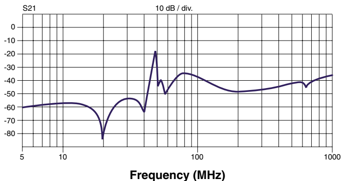
Isolation (TYP)
