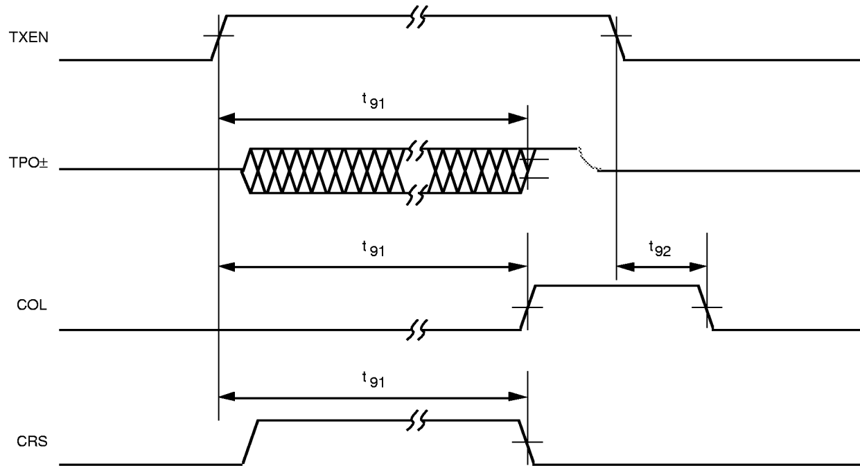
Figure 29. Jabber Timing
