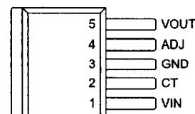
TO-263-5 (Front View) TD Package
