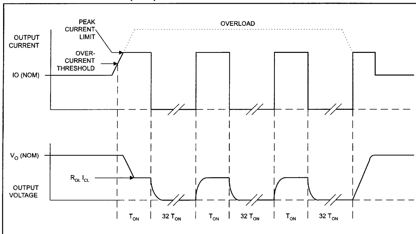
Figure 1. UCC383 Short Circuit Timing
