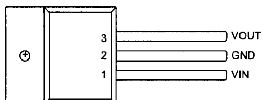
TO-220-3 (Front View) T Package
