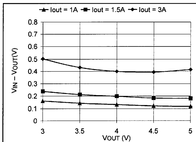
Figure 3. Typical Dropout Voltage vs. I_{OUT} and V_{OUT}
