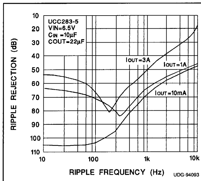
Figure 7. Ripple rejection vs. frequency.
