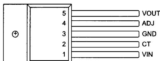
TO-220-5 (Front View) T Package
