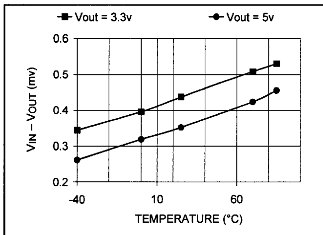
Figure 4. Typical dropout voltage vs. case temperature with a 3A load
