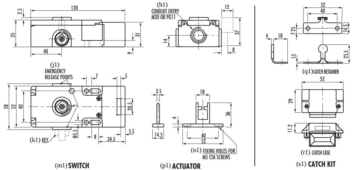
(m1) SWITCH
