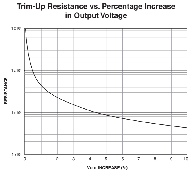
Figure 7. USQ-1.2 Trim-Up Resistance vs. % Increase V_{OUT}
