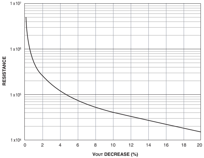
Figure 13. USQ-1.5 to USQ-3.3 Trim-Down Resistance vs. % Decrease Vout
