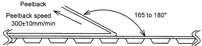
Fig. 8 Test method
