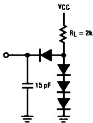
Load Circuit 1
