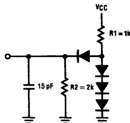
Load Circuit 2
