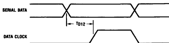
FIGURE 11. Data Clock and Serial Data Timing
