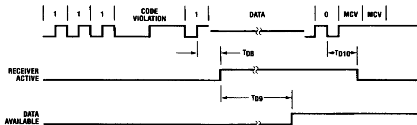
FIGURE 10. Message Timing
