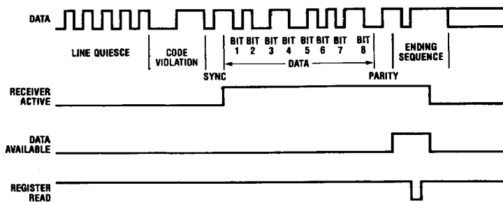
FIGURE 4a. Single Byte (8-Bit) Message
