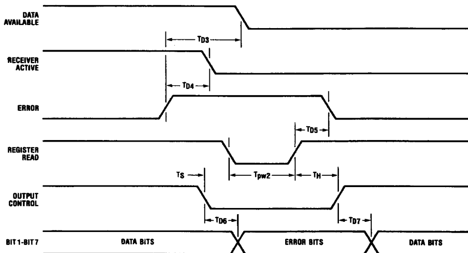
FIGURE 9. Error Sequence Timing
