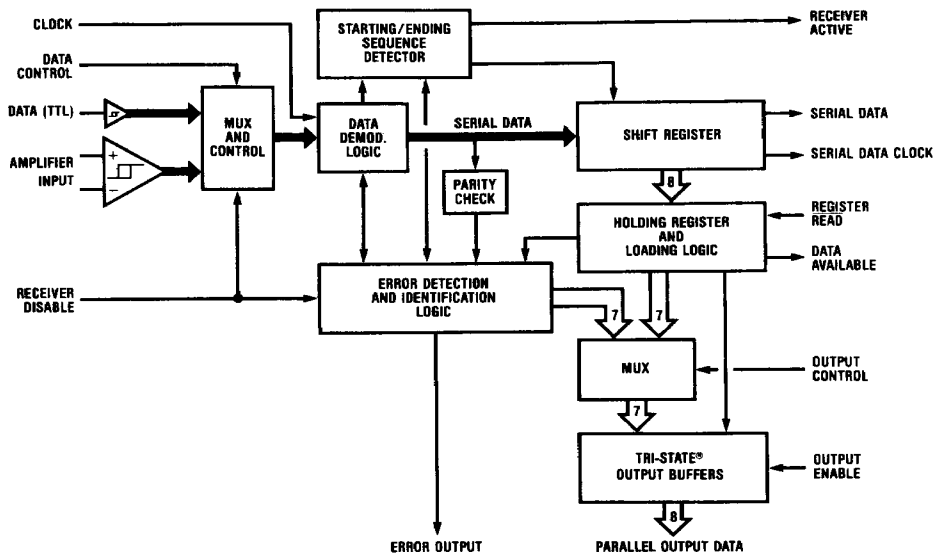
FIGURE 2. DP8343/NS32443 Biphase Receiver
