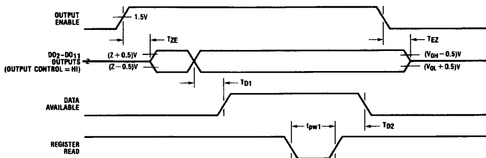
FIGURE 8. Data Sequence Timing
