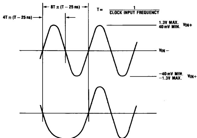
FIGURE 12. Data Waveform Constraints: Amplifier Inputs
