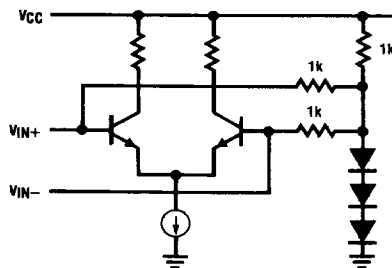
FIGURE 14. Equivalent Circuit for DP8343/NS32443 Input Amplifier
