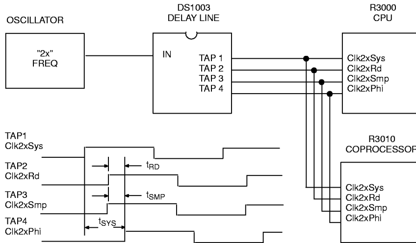
TYPICAL APPLICATION Figure 5
