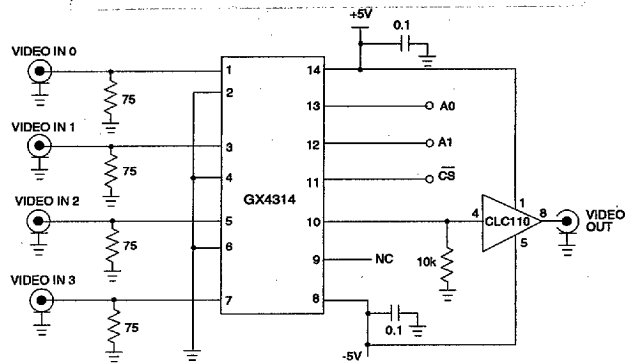
Fig. 7 Test Circuit
