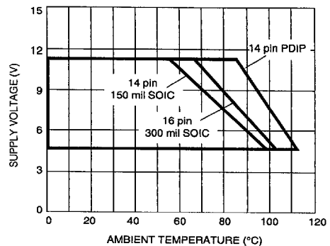
Fig. 6 Safe Operating Area for GX4314 (All packages)
