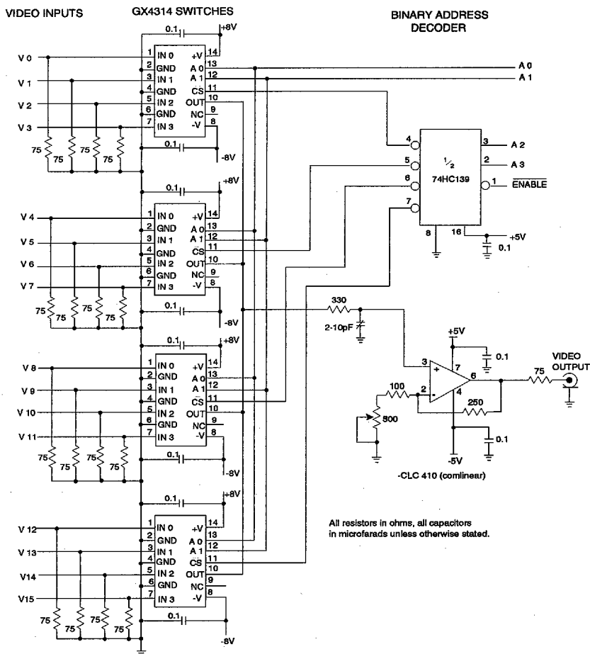
Fig. 8 16 x 1 Video Multiplexer Circuit
