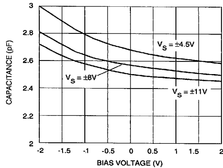
Fig. 4 Output Capacitance
