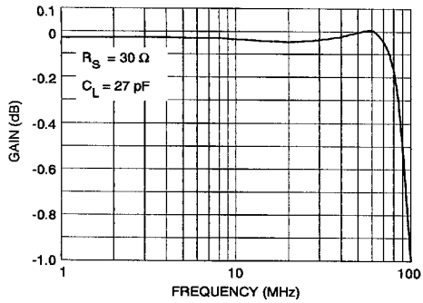
Fig. 1 Flattened Frequency Response
