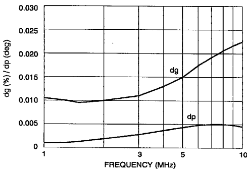
Fig. 5 Differential Gain & Phase
