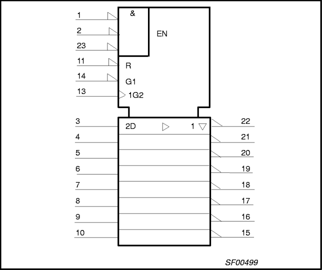
IEC/IEEE SYMBOL – 74F826
