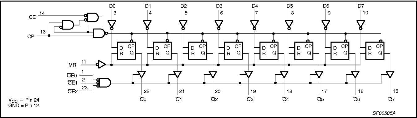
LOGIC DIAGRAM FOR 74F826
