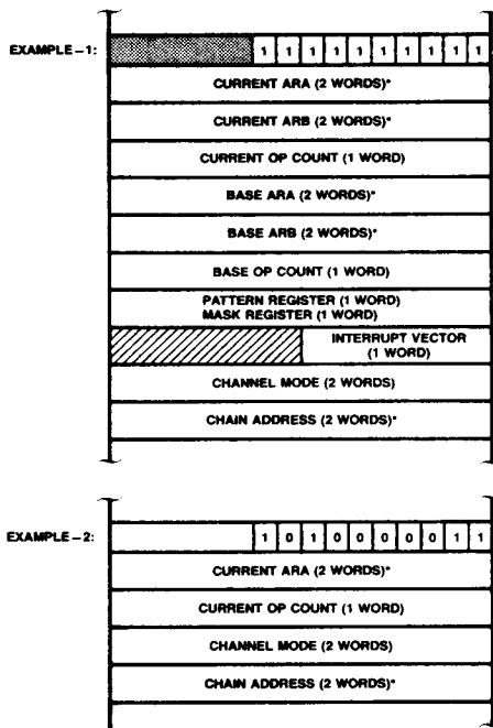
Figure 12. Examples of Chain Control Table
