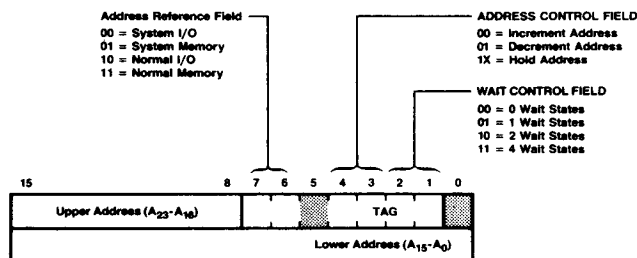
Figure 4. Address Registers A and B
