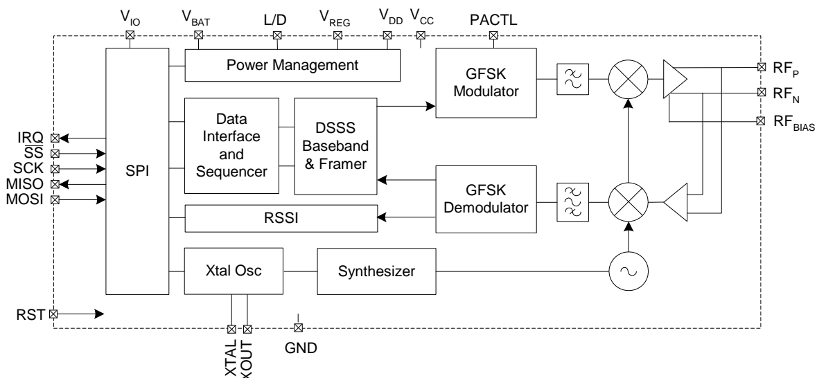
CYRF6936 Simplified Block Diagram
