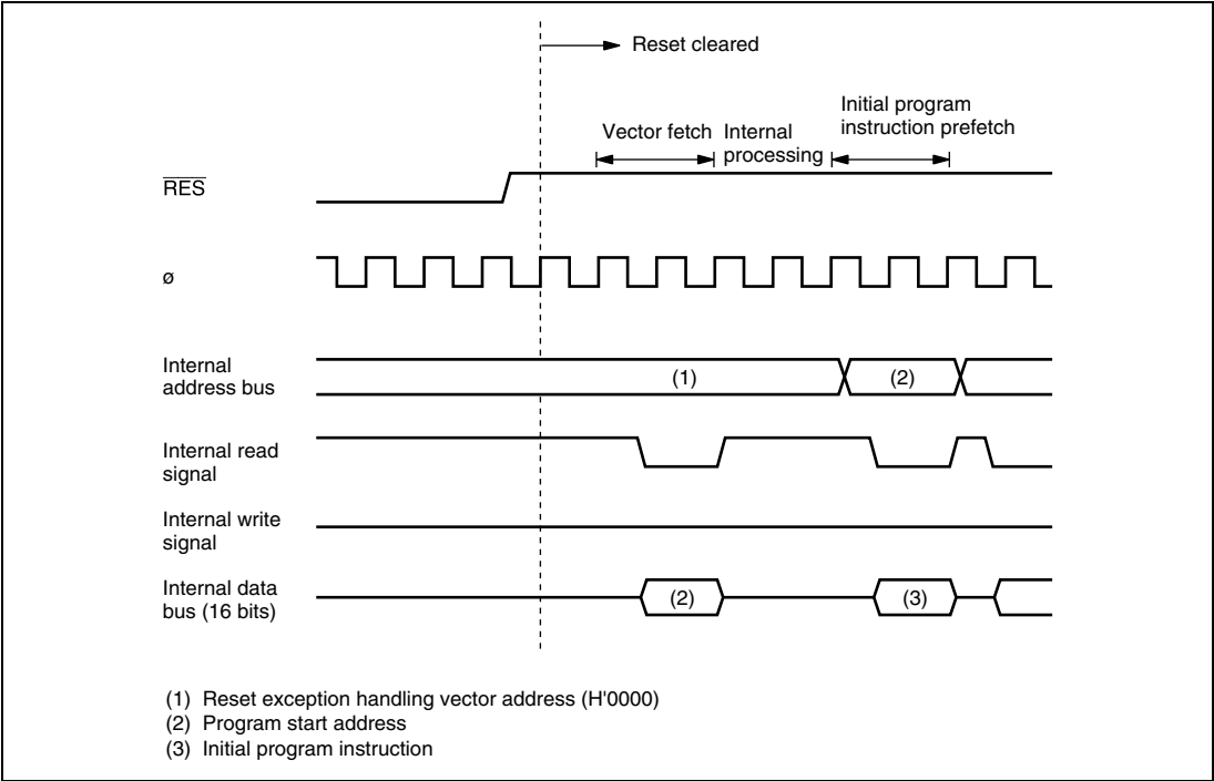
Figure 3.1 Reset Sequence
