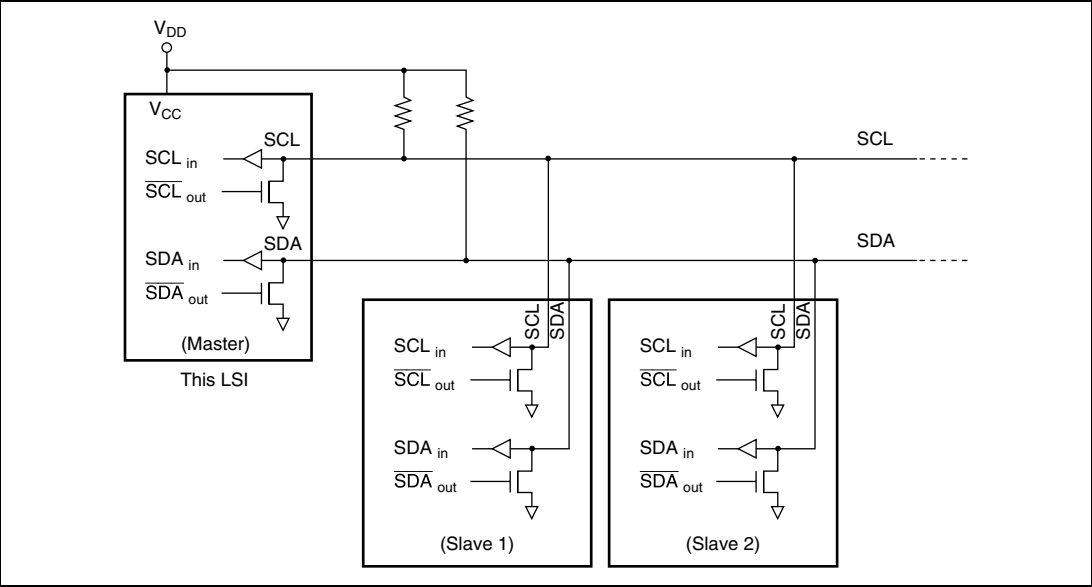
Figure 15.2 I²C Bus Interface Connections (Example: This LSI as Master)
