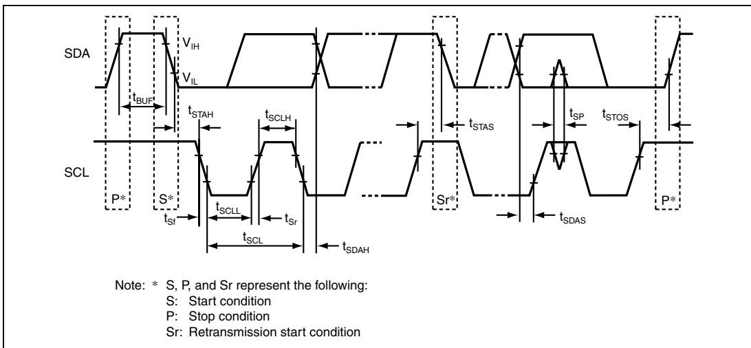
Figure 20.4 I²C Bus Interface Input/Output Timing
