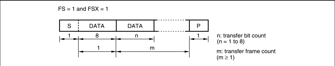
Figure 15.10 I²C Bus Data Format (Serial Format)
