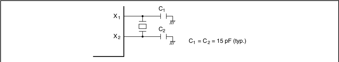
Figure 5.8 Typical Connection to 32.768-kHz Crystal Resonator
