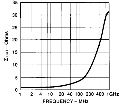
Output Impedance
