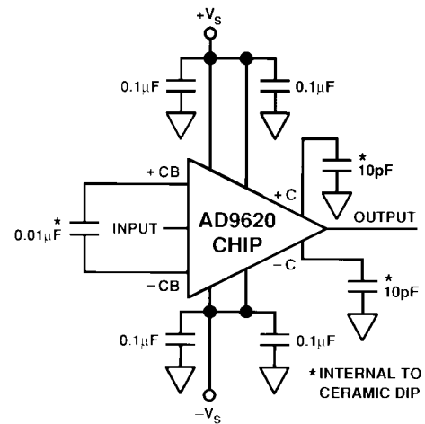
AD9620 Bonding Diagram
