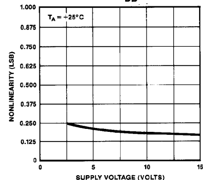
NONLINEARITY vs V_{DD}
