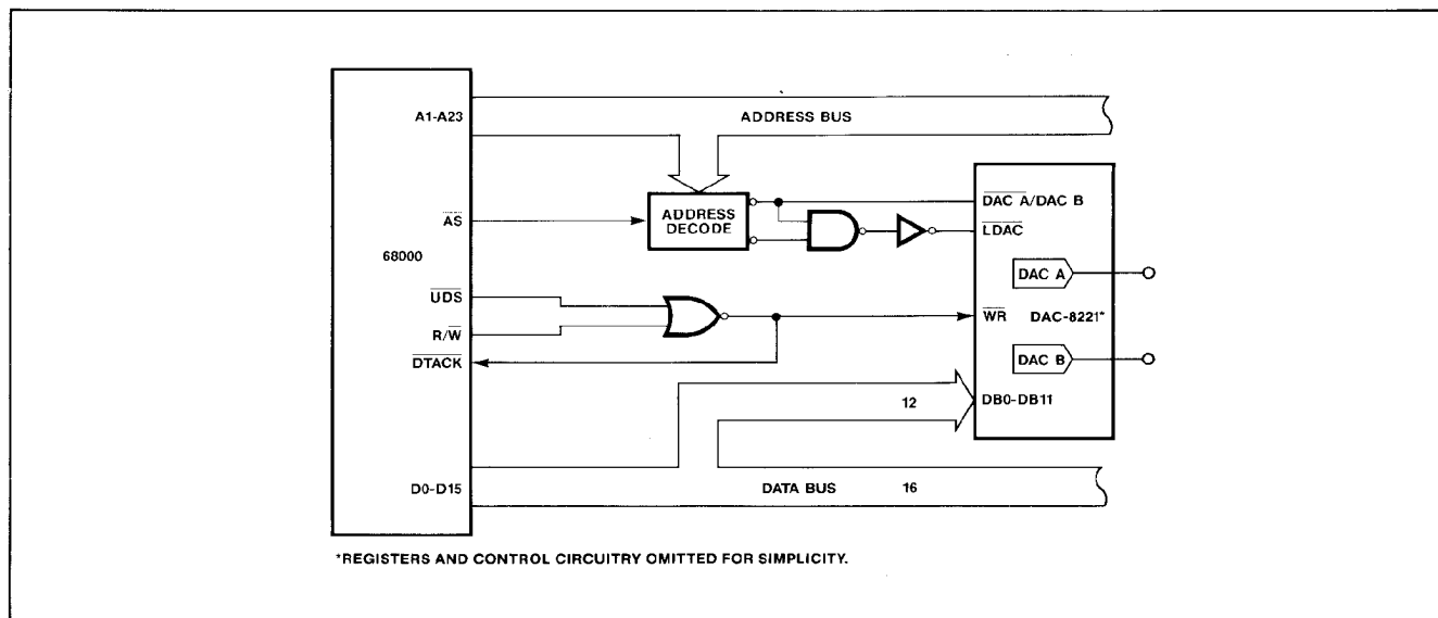
FIGURE 10: DAC-8221 To 68000 Interface
