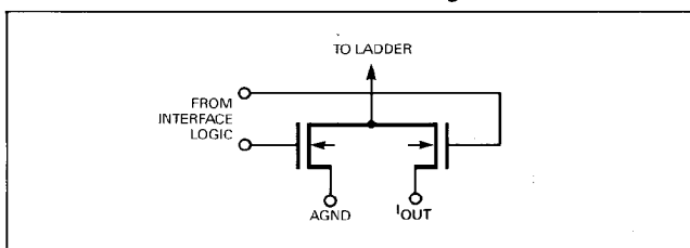
FIGURE 2: N-Channel Current Steering Switch
