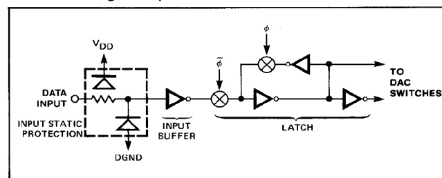
FIGURE 3: Digital Input Structure For One Bit
