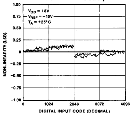
NONLINEARITY vs CODE (DAC A & B ARE SUPERIMPOSED)
