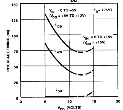
INTERFACE TIMING vs V_{DD}
