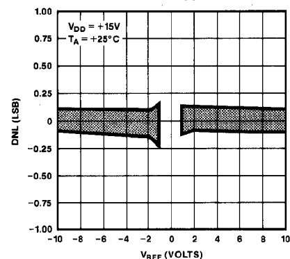
DIFFERENTIAL NONLINEARITY vs V_{REF}
