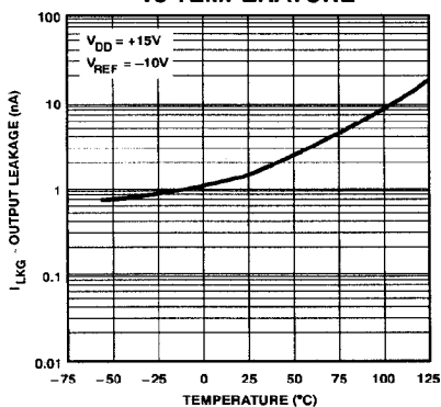
OUTPUT LEAKAGE CURRENT vs TEMPERATURE
