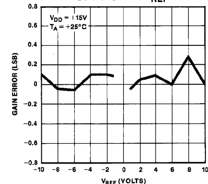
ABSOLUTE GAIN ERROR CHANGE vs V_{REF}
