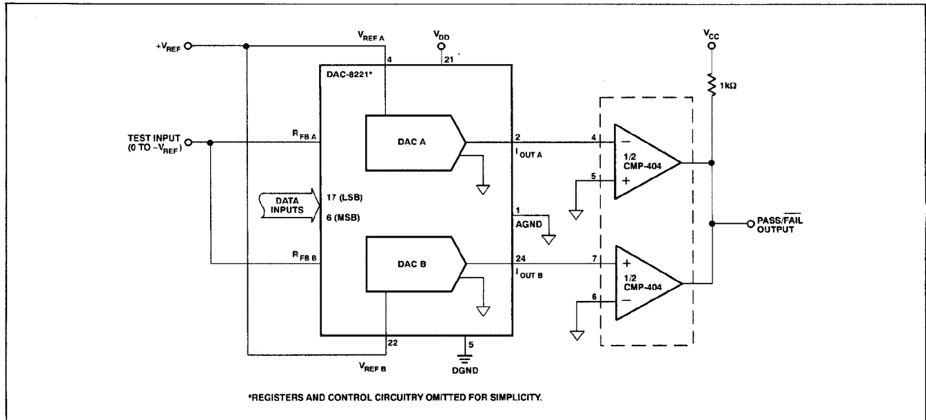
FIGURE 8: Digitally-Programmable Window Detector (Upper/Lower Limit Detector)
