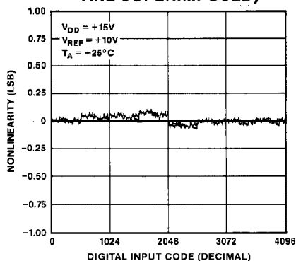
CHANNEL-TO-CHANNEL MATCHING (DAC A & B ARE SUPERIMPOSED)
