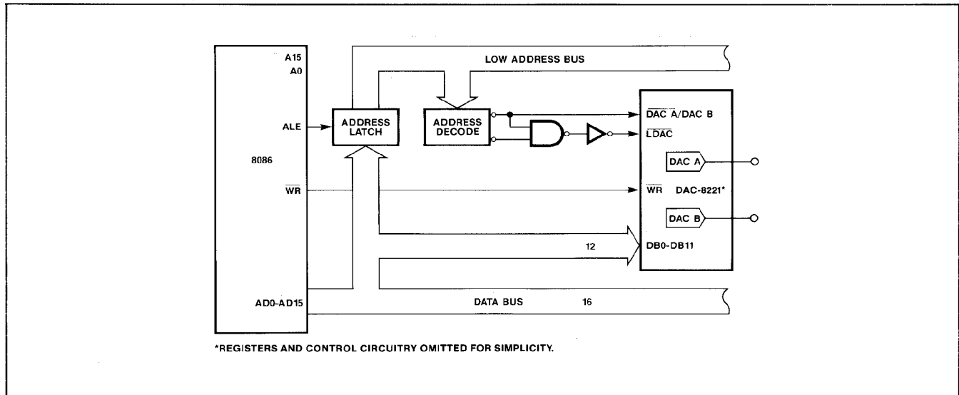
FIGURE 9: DAC-8221 To 8086 Interface
