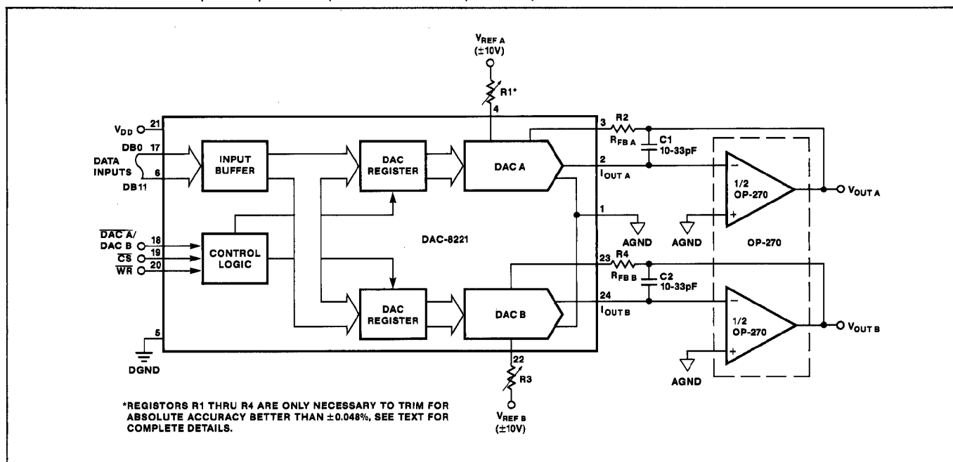
FIGURE 4: Dual DAC Unipolar Operation (2-Quadrant Multiplication)
