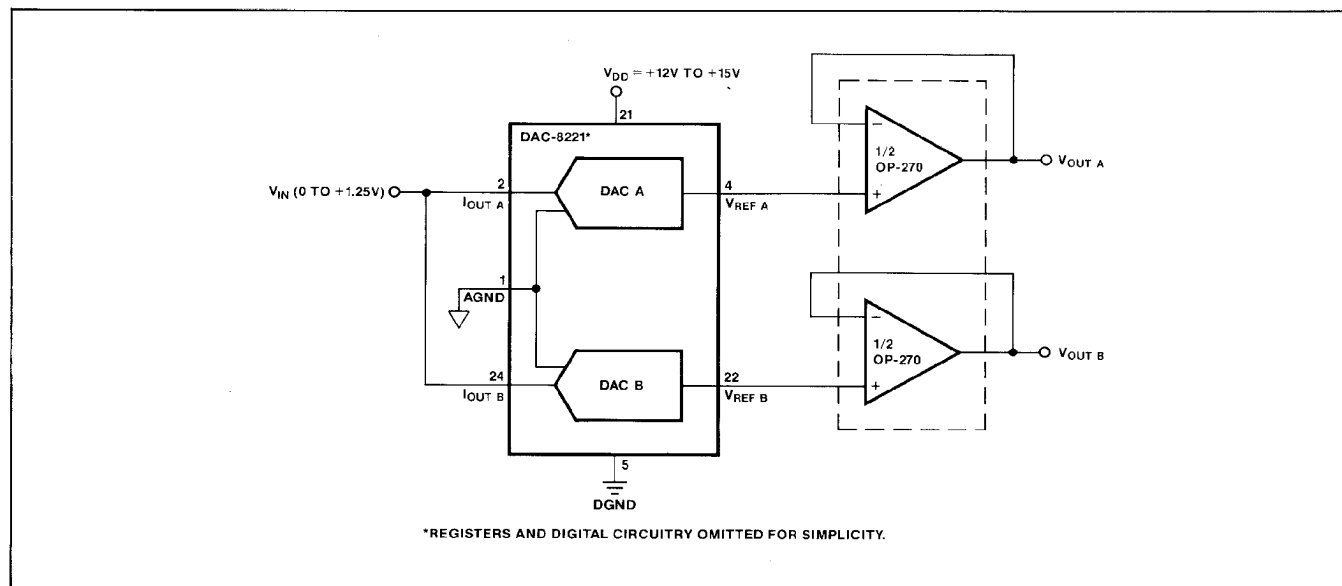
FIGURE 7: Single Supply Operation (Voltage Switching Mode)
