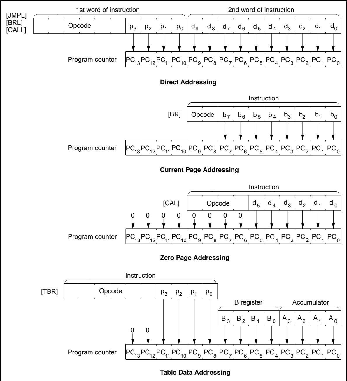
Figure 76 ROM Addressing Modes
