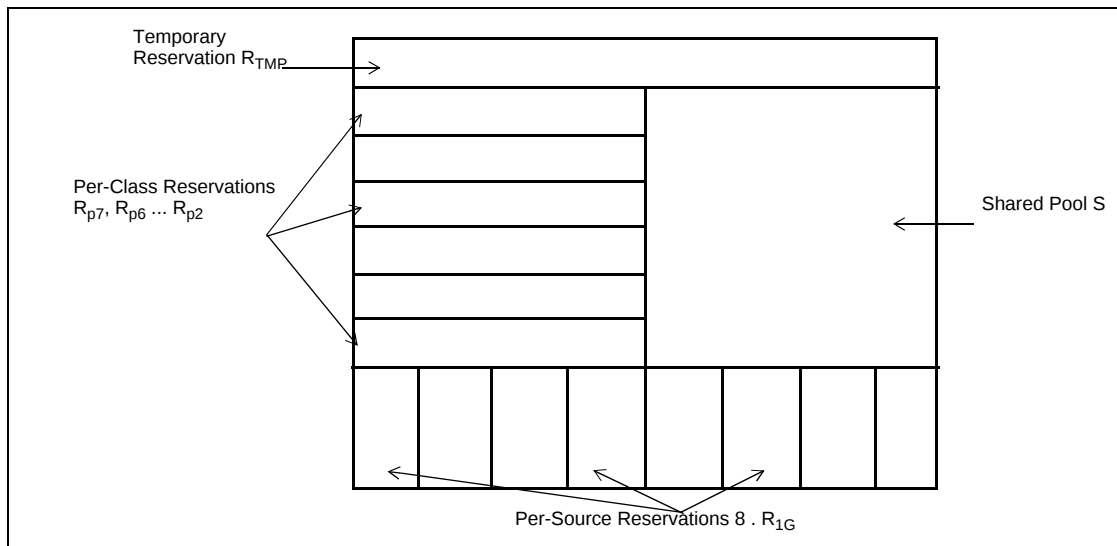
Figure 6 - Buffer Partition Scheme Used in the MVTX2801AG
