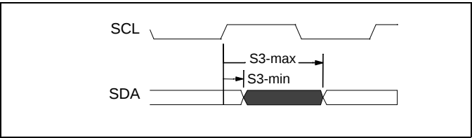
Figure 22 - I 2 C Output Delay Timing
