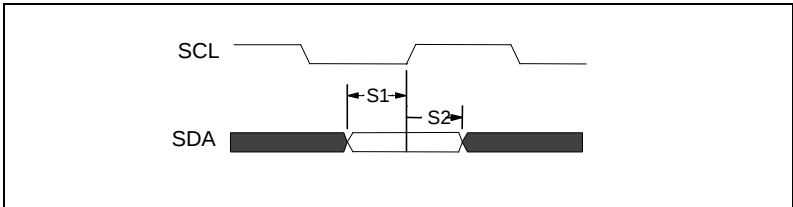
Figure 21 - I 2 C Input Setup Timing
