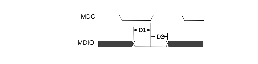
Figure 19 - MDIO Input Setup and Hold Timing
