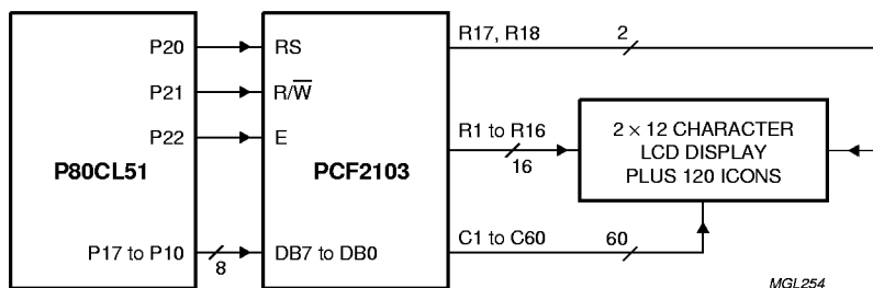
Fig.25 Direct connection to 8-bit microcontroller; 8-bit bus.
