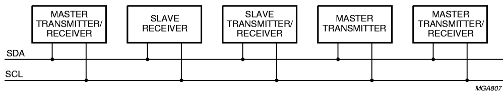
Fig.15 System configuration.
