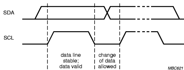
Fig.16 Bit transfer.
