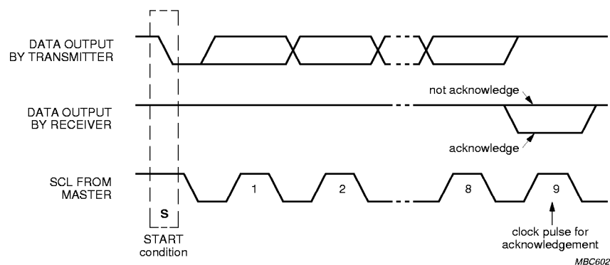
Fig.18 Acknowledgement on the I 2 C-bus.
