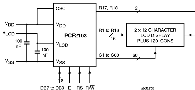
Fig.27 Application example using parallel interface.
