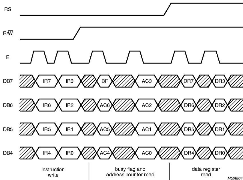
Fig.11 4-bit transfer example.
