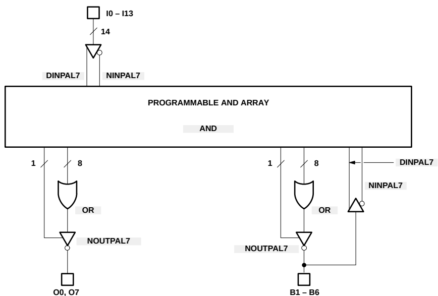
PLUS20L8
