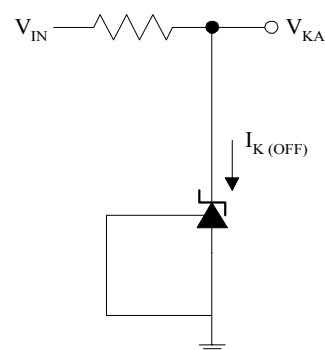
Figure 1c. Test Circuit 3
