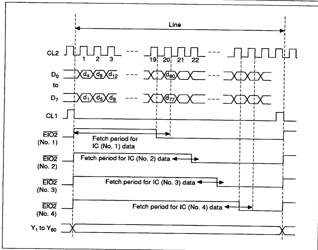
Figure 5 Operation Timing (4-Bit Fetch Mode)
