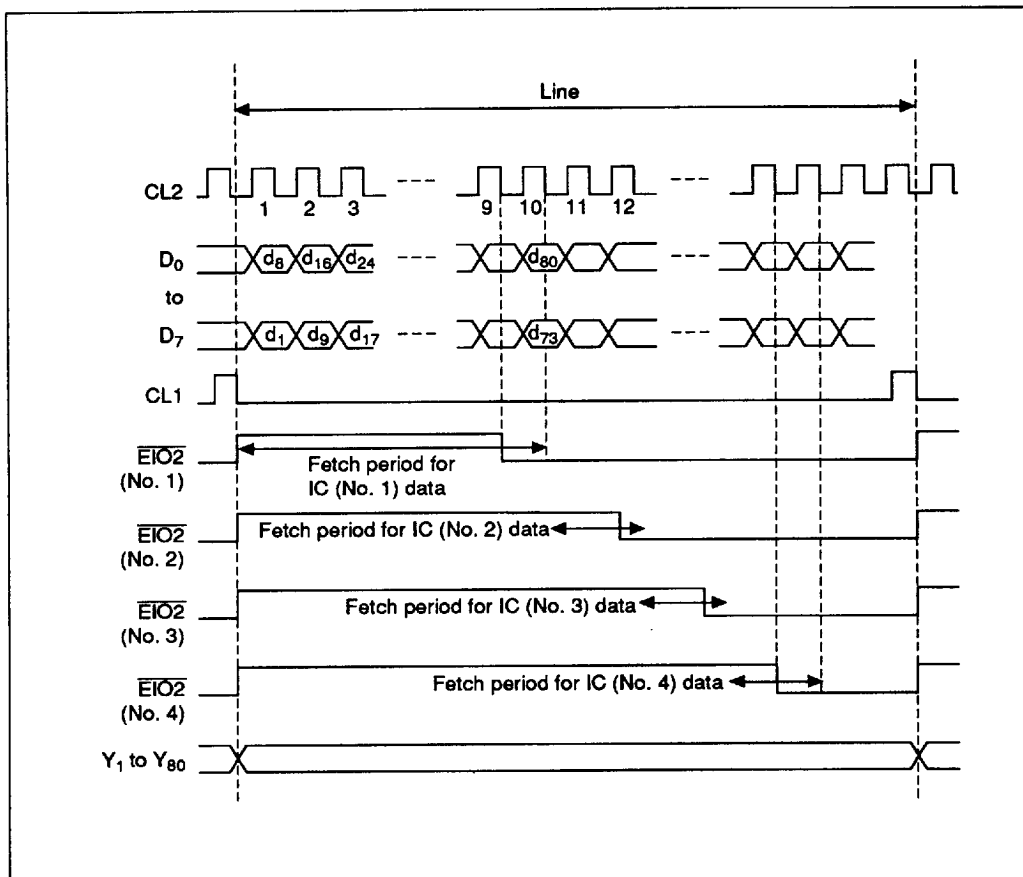
Figure 6 Operation Timing (8-Bit Fetch Mode)
