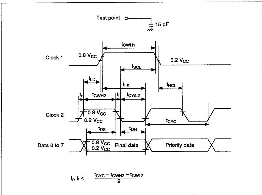
Figure 4 AC Characteristic Waveforms
