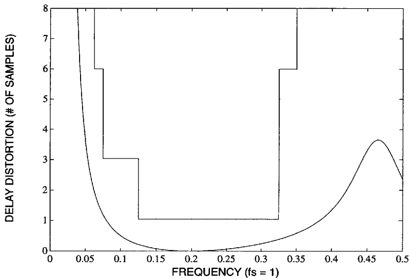
Figure 15. A/D or D/A Path Group Delay Distortion (HPF Enabled)
