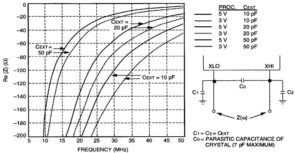
Figure 27. Negative Resistance of Crystal Oscillator Circuit, V_{DD} = 4.75 V
