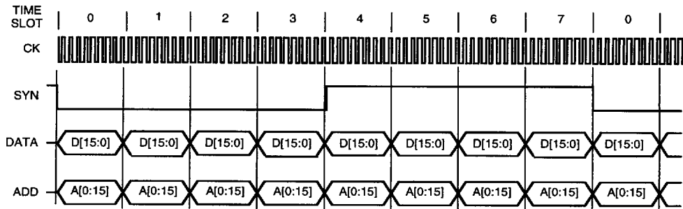
Figure 21. Multiprocessor Frame Timing
