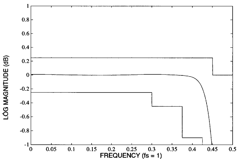
Figure 9. A/D or D/A Path Frequency Response over 0.5 f_s Bandwidth (HPF Disabled)
