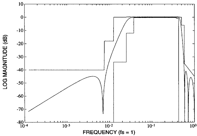
Figure 12. A/D or D/A Path Frequency Response over f_s Bandwidth (HPF Enabled)
