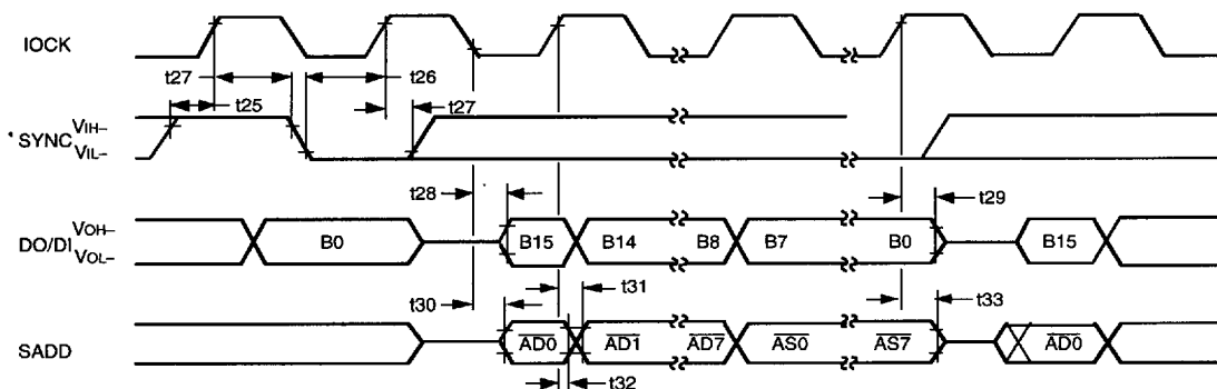
Figure 40. SIO Multiprocessor Timing Diagram
