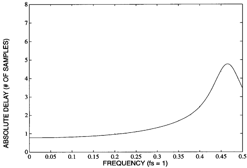
Figure 10. A/D or D/A Path Absolute Group Delay (HPF Disabled)
