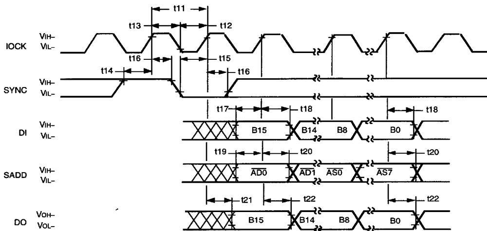
Figure 38. Serial Input/Output Timing Diagram
