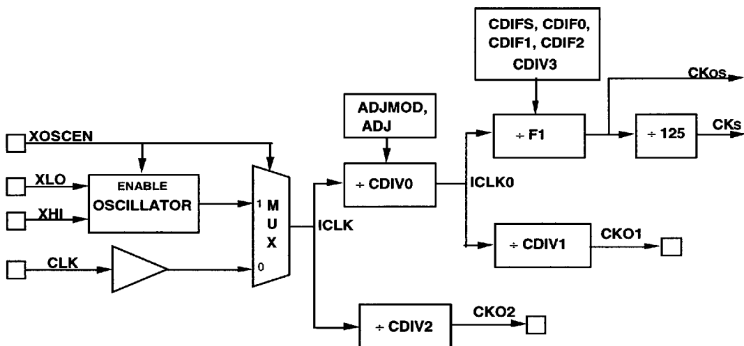
Figure 17. Clock Generation
