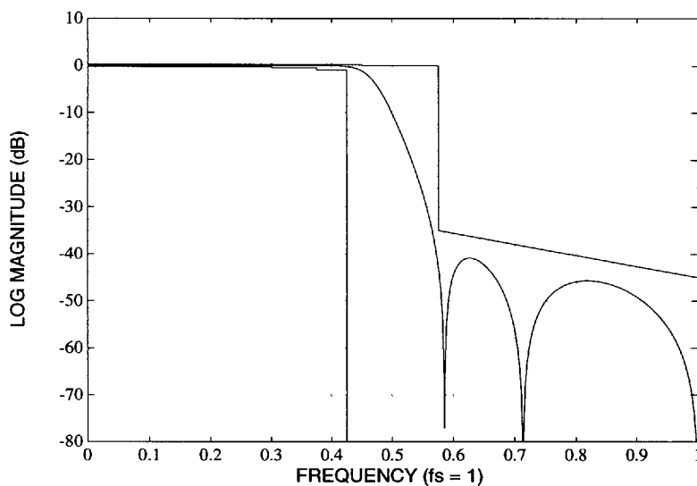
Figure 8. A/D or D/A Path Frequency Response over f_s Bandwidth (HPF Disabled)
