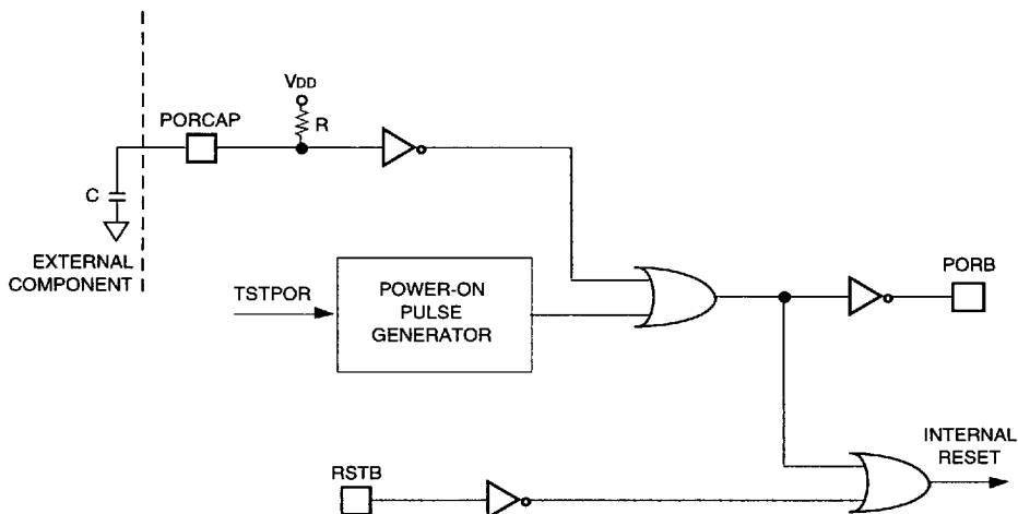
Figure 16. Power-On Reset Diagram
