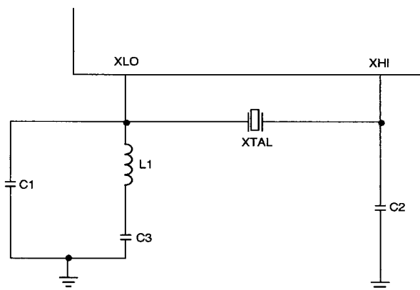
Figure 31. Third Overtone Crystal Configuration
