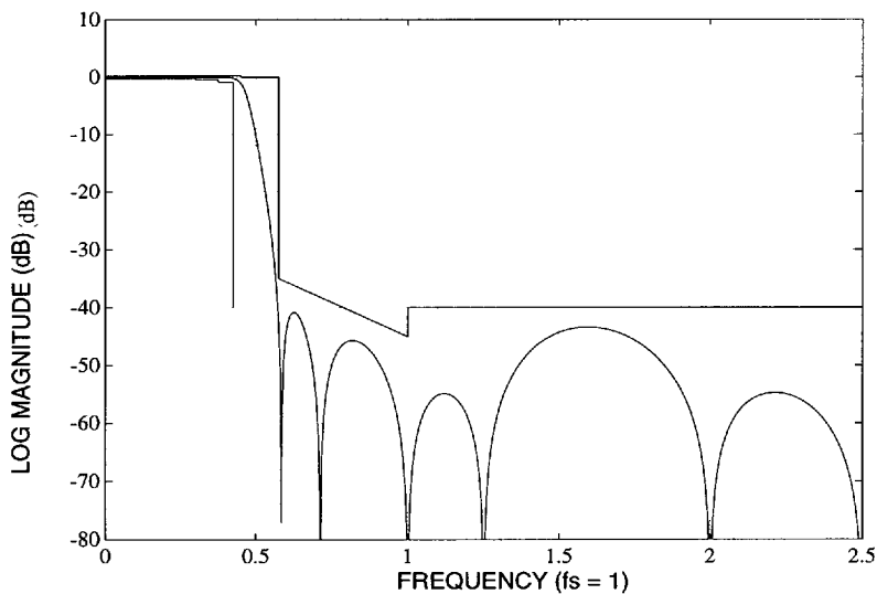
Figure 7. A/D or D/A Path Frequency Response over 2.5 f_s Bandwidth (HPF Disabled)
