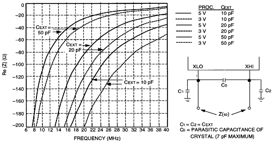
Figure 28. Negative Resistance of Crystal Oscillator Circuit, V_{DD} = 3.0 V
