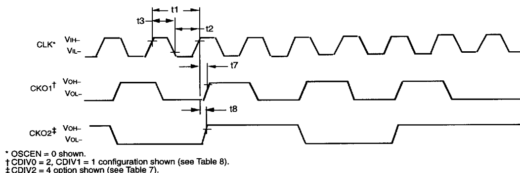
Figure 35. Clock Timing Diagram
