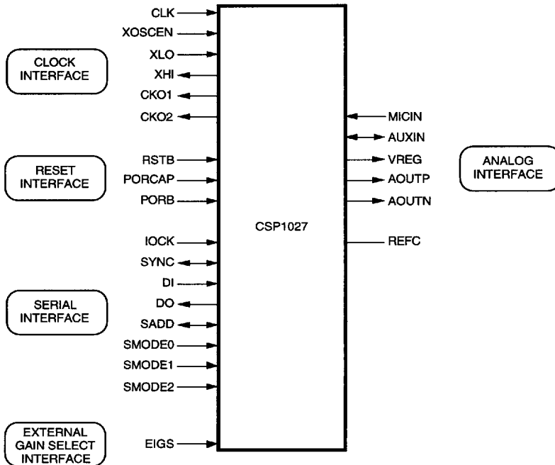
Figure 23. CSP1027 Pinout by Interface
