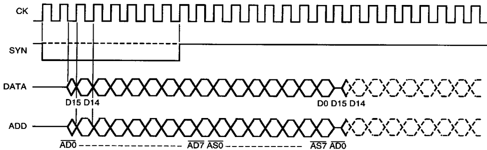
Figure 22. Multiprocessor Time-Slot Timing
