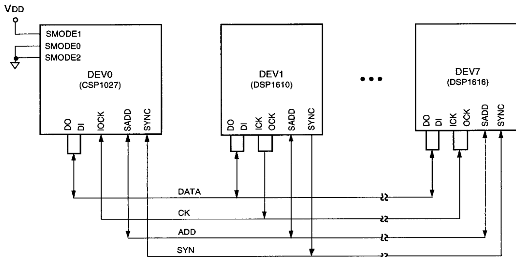
Figure 20. Multiprocessor Communication and Connections
