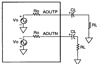
E. DUAL SINGLE-ENDED
