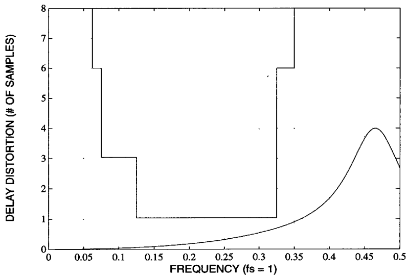
Figure 11. A/D or D/A Path Group Delay Distortion (HPF Disabled)
