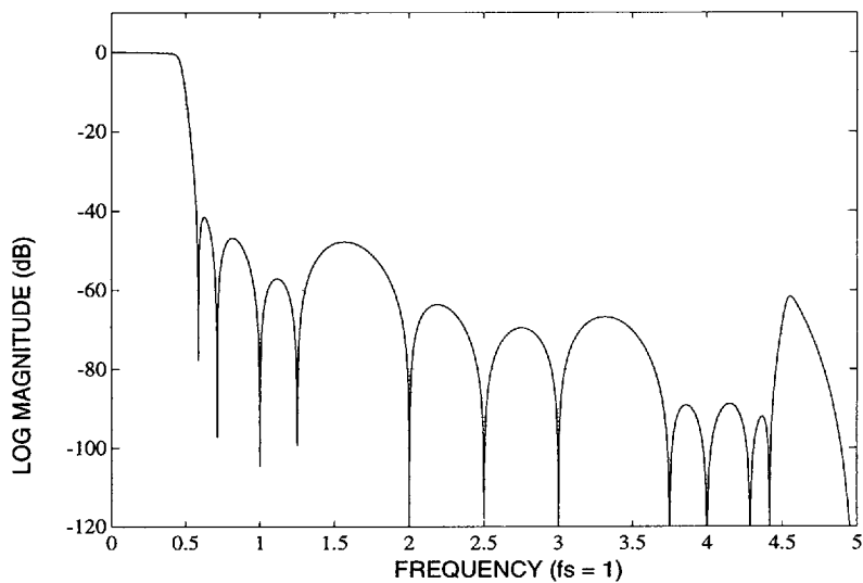
Figure 6. A/D or D/A Path Frequency Response over 5 f_s Bandwidth (HPF Disabled)
