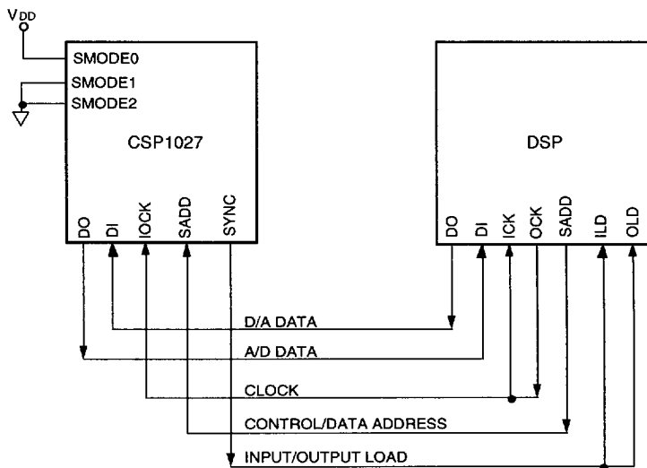
Figure 19. Active Communication and Connections
