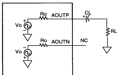
C. SINGLE-ENDED, AOUTP
