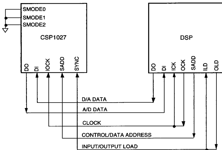
Figure 18. Passive Communication and Connections
