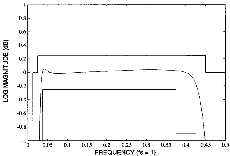
Figure 13. A/D or D/A Path Frequency Response over 0.5 f_s Bandwidth (HPF Enabled)
