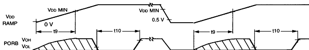
Figure 36. Power-On Reset Timing Diagram
