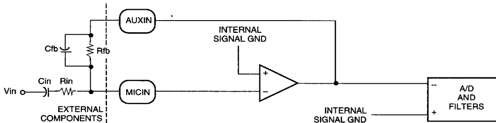
Figure 5. CSP1027 A/D Path in the External Gain Select Mode (EIGS = 1)
