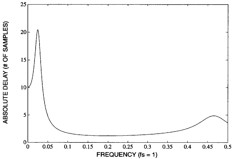
Figure 14. A/D or D/A Path Absolute Group Delay (HPF Enabled)
