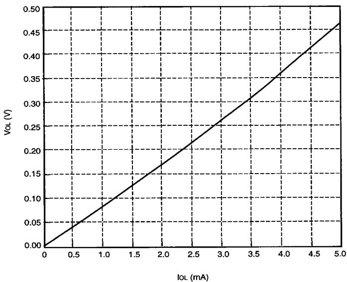
Figure 34. Plot of V_{OL} vs. I_{OL} Under Typical Operating Conditions
