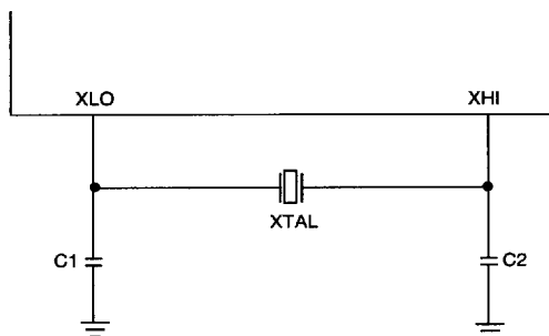
Figure 26. Fundamental Crystal Configuration
