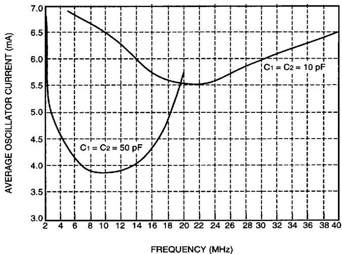
Figure 29. Typical Supply Current of Crystal Oscillator Circuit, V_{DD} = 5.0\text{ V} , 25\text{ }^{\circ}\text{C}
