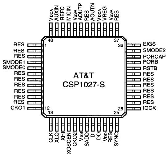
Figure 2. 48-Pin EIAJ Thin Quad Flat Pack (TQFP) Pin Diagram
