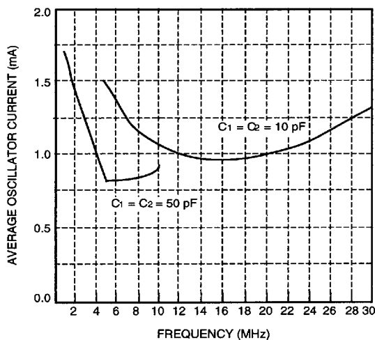
Figure 30. Typical Supply Current of Crystal Oscillator Circuit, V_{DD} = 3.3\text{ V} , 25\text{ }^{\circ}\text{C}
