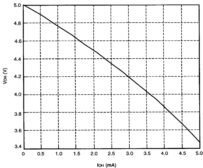
Figure 33. Plot of V_{OH} vs. I_{OH} Under Typical Operating Conditions
