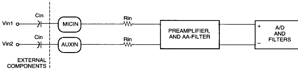
Figure 4. CSP1027 A/D Path when in the Preamplifier Mode (EIGS = 0)
