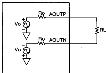
A. FULLY DIFFERENTIAL
