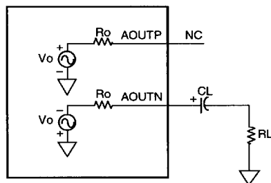
D. SINGLE-ENDED, AOUTN
