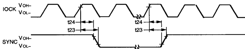
Figure 39. Serial I/O Active Mode Timing Diagram
