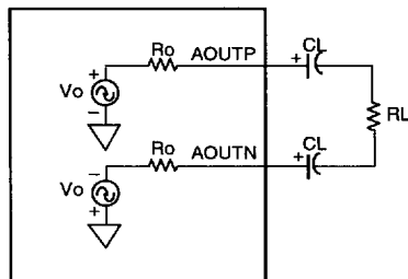
B. FULLY DIFFERENTIAL, WITH CAPACITIVE COUPLING
