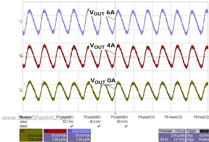
FIGURE 13. 2.5V OUTPUT RIPPLE
