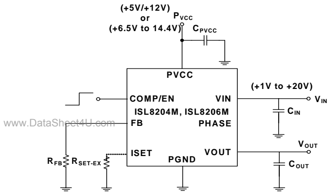
FIGURE 16. WIDE INPUT VOLTAGE APPLICATION SCHEMATIC
