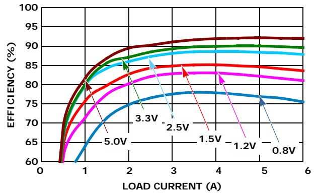
FIGURE 4. EFFICIENCY vs LOAD CURRENT ( 12\text{V}_{IN} )
