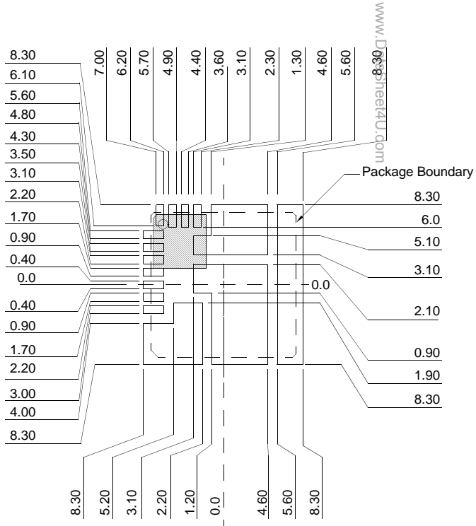
TYPICAL RECOMMENDED LAND PATTERN
