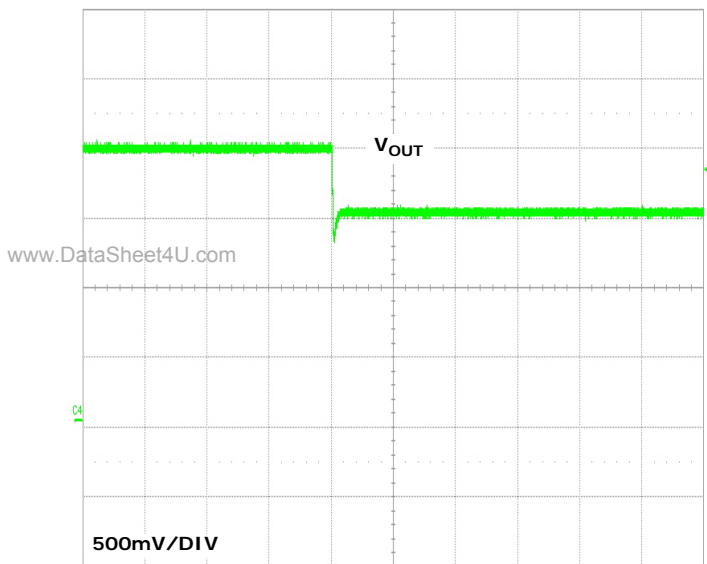
FIGURE 22. PRE-BIASED START-UP - OVERCHARGED
