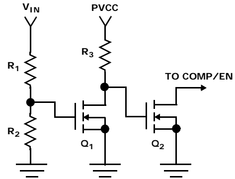
FIGURE 24. SEQUENCE CIRCUIT
