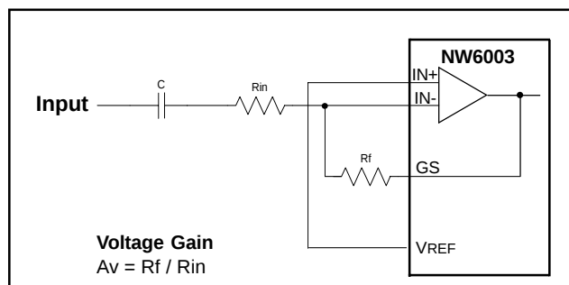
Figure-4. Single-ended Input Gain Control Circuit
