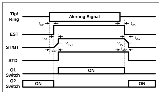
Figure-8. Guard Time Waveform
