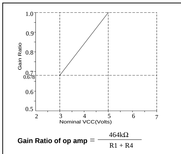
Figure-12. Gain Ratio as a Function of Nominal VCC
