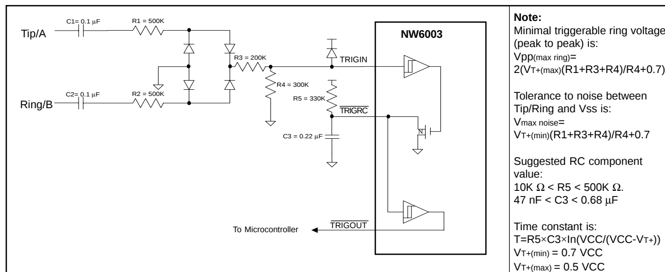
Figure-6. CLIP/CID Call Arrival Detection Circuit
