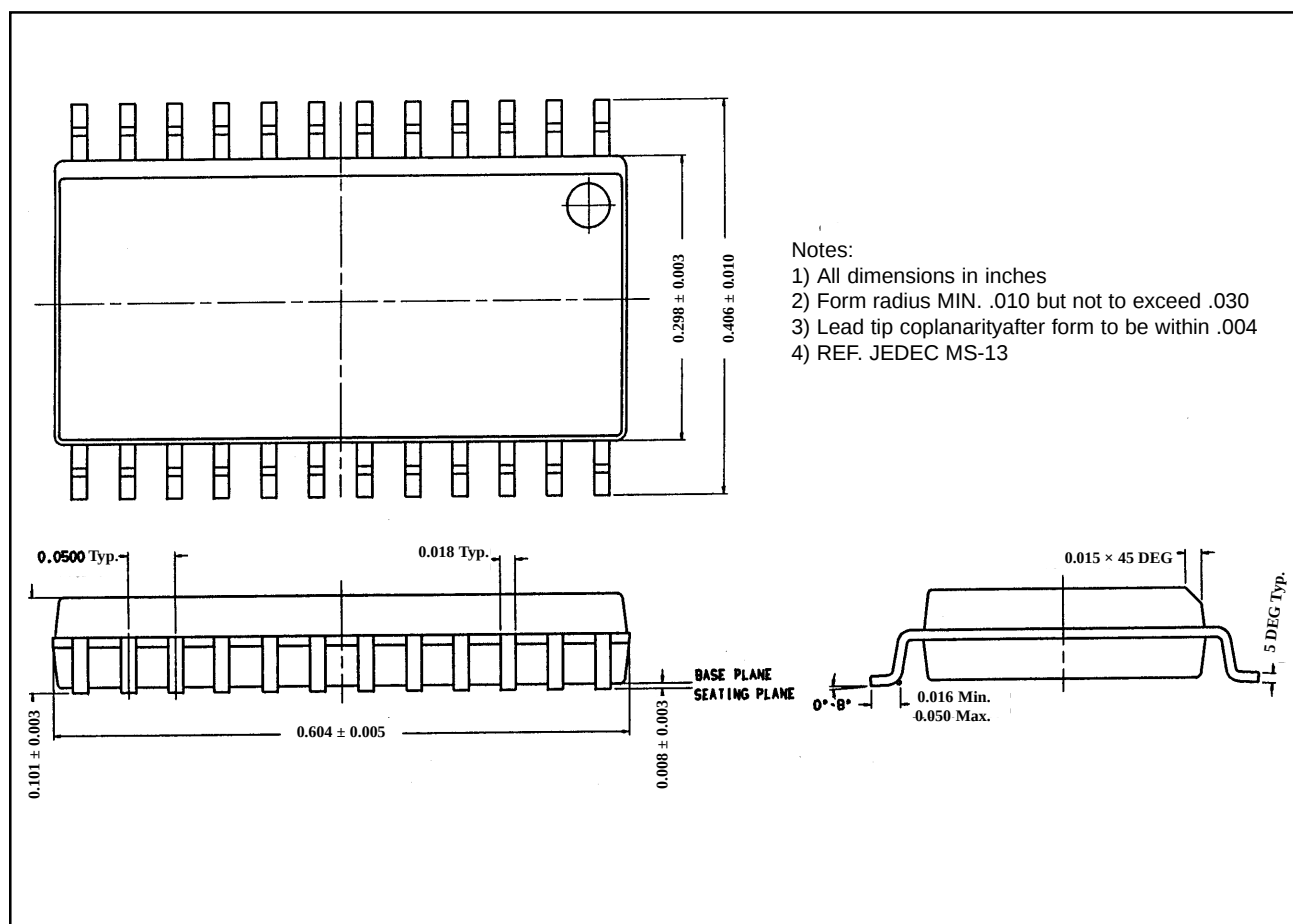
Figure-25. NW6003-XS 24 Pin SOIC Package Diagram
