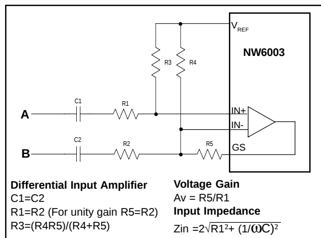
Figure-3. Differential Input Gain Control Circuit
