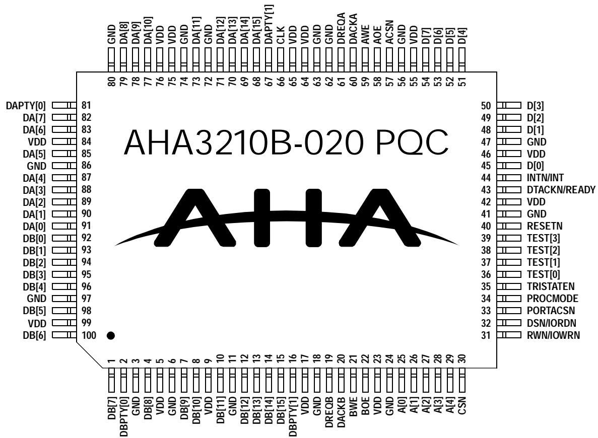
Figure 11: Pinout Diagram
