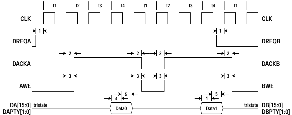
Figure 24: DMA Slave Transfer Timing for Data Into Port A,B
