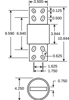
Fig. 3: 1200 Amp Range
