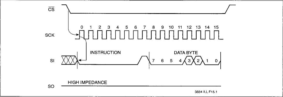
Figure 6. Write Status Register Operation Sequence
