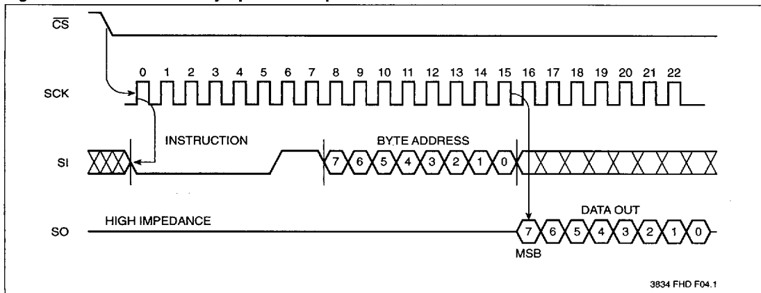
Figure 1. Read E 2 PROM Array Operation Sequence
