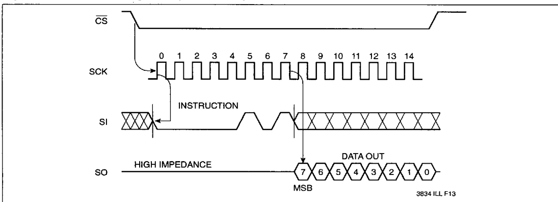
Figure 2. Read Status Register Operation Sequence
