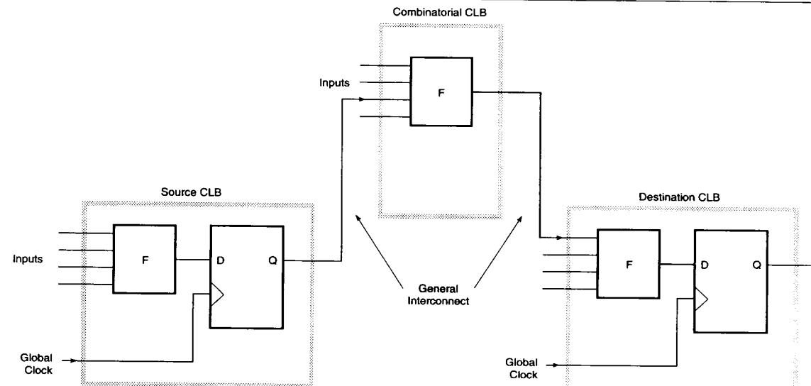
Figure 18. Typical Logic Path
