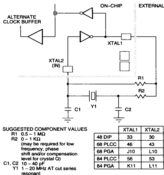
Figure 10. Crystal Oscillator
