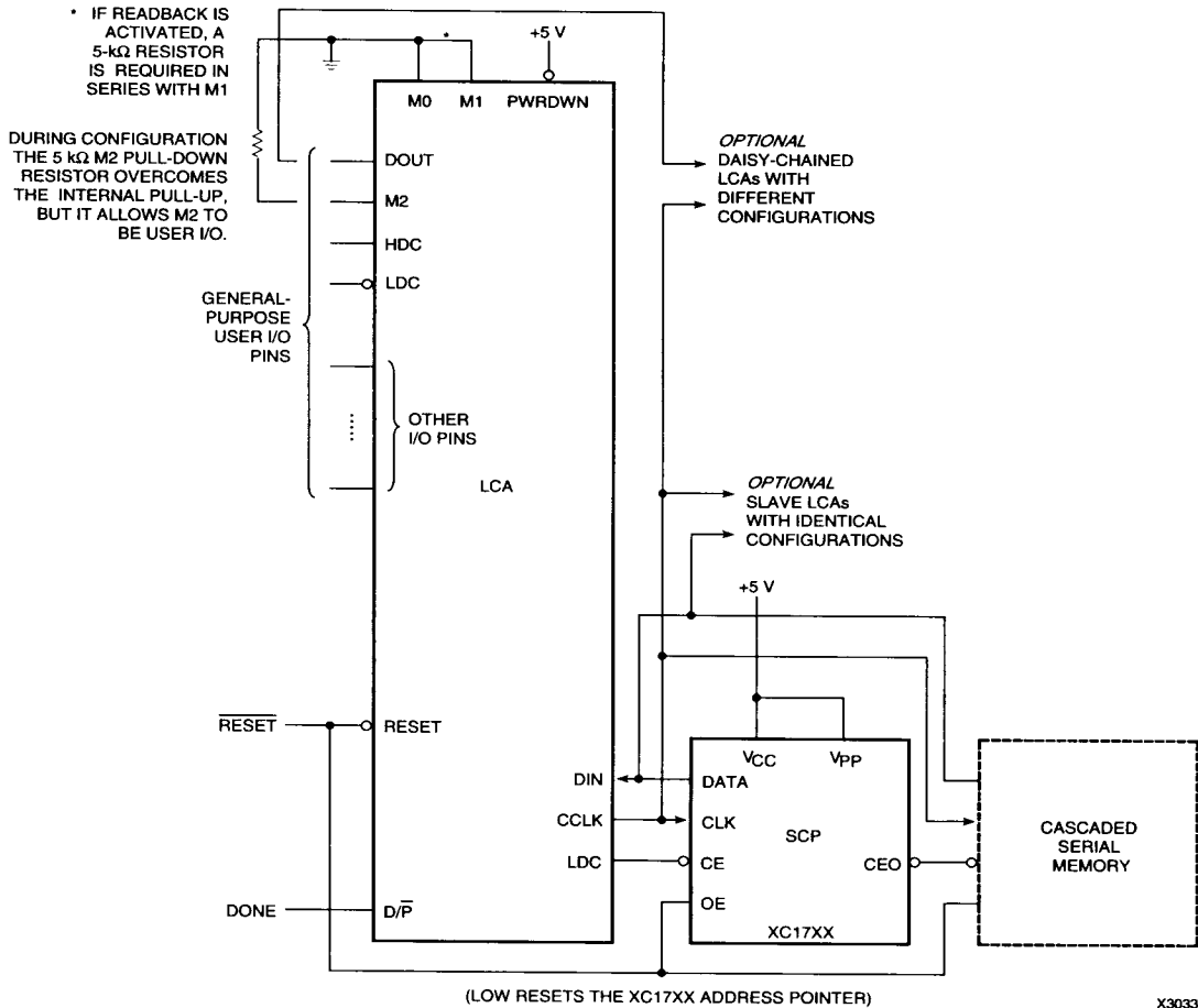
Figure 13. Master Serial Mode
