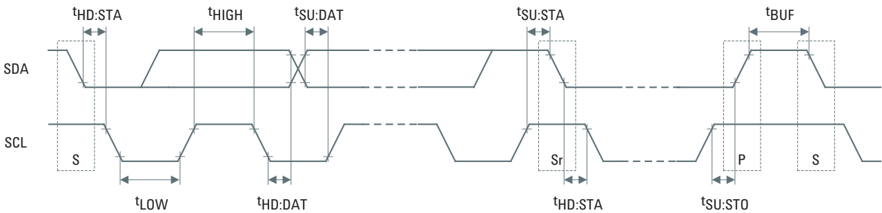
Figure 2. Serial Interface Bus Timing Waveforms
