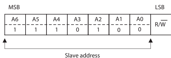
Figure 9. Slave Addressing
