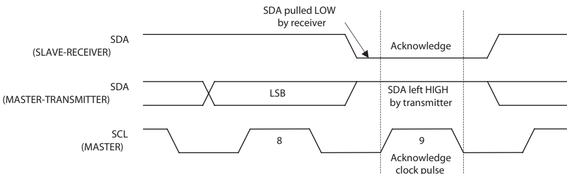
Figure 7. Slave-Receiver Acknowledge
